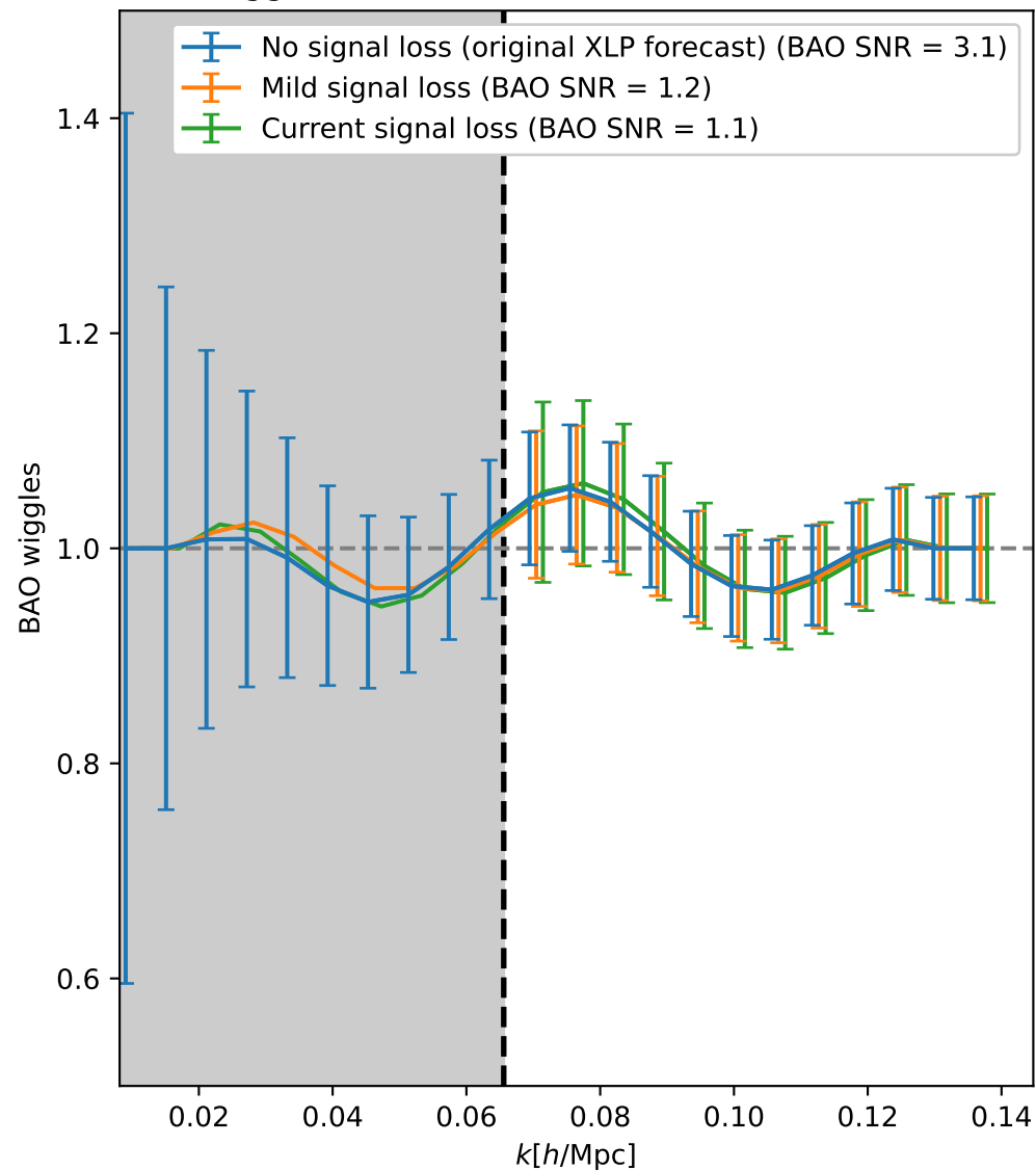
BAO wiggles (DESI-cross at z=0.61 , 880hrs total time)
