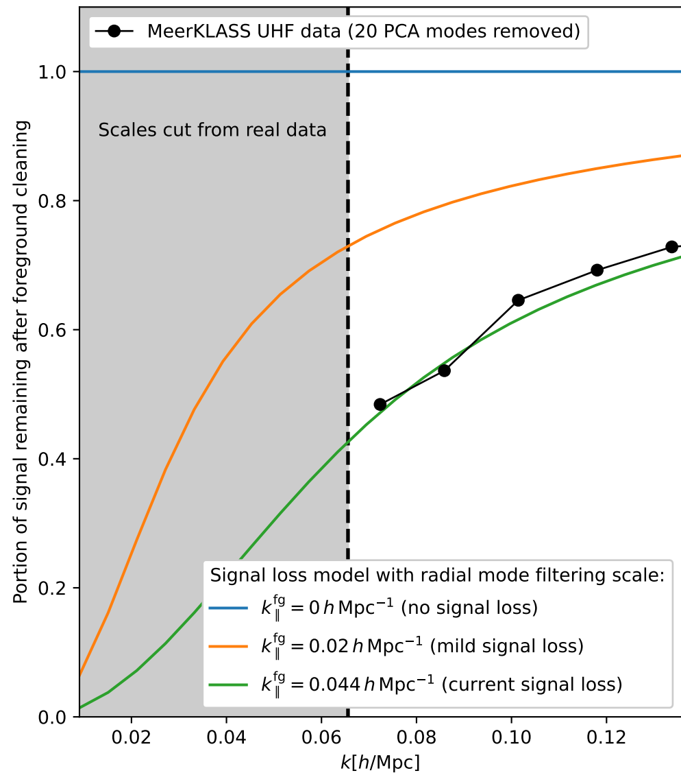
Estimate of signal loss using foreground transfer function \tau(k)
