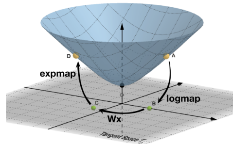
Figure 1: Illustration of Lorentz model and tangent space operations. Reproduced from Chen et al. [8].
