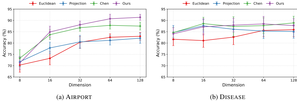
Figure 3: Classification accuracy and standard deviation as a function of embedding dimensionality on the Airport and Disease datasets.
