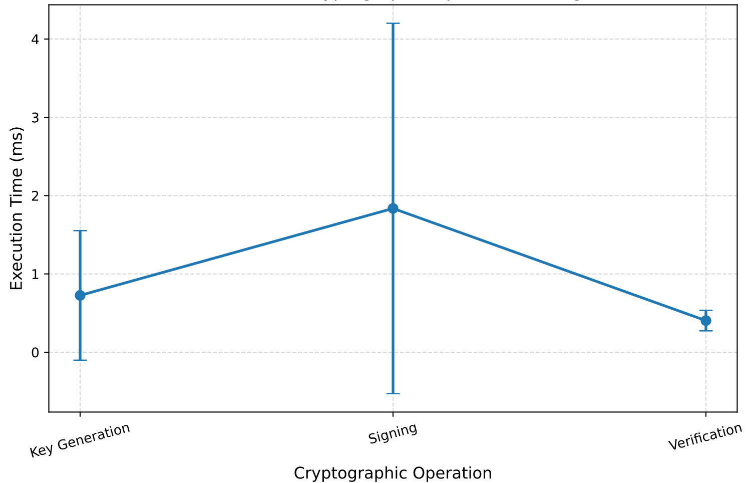
ML-DSA-65 Cryptographic Operation Timing
