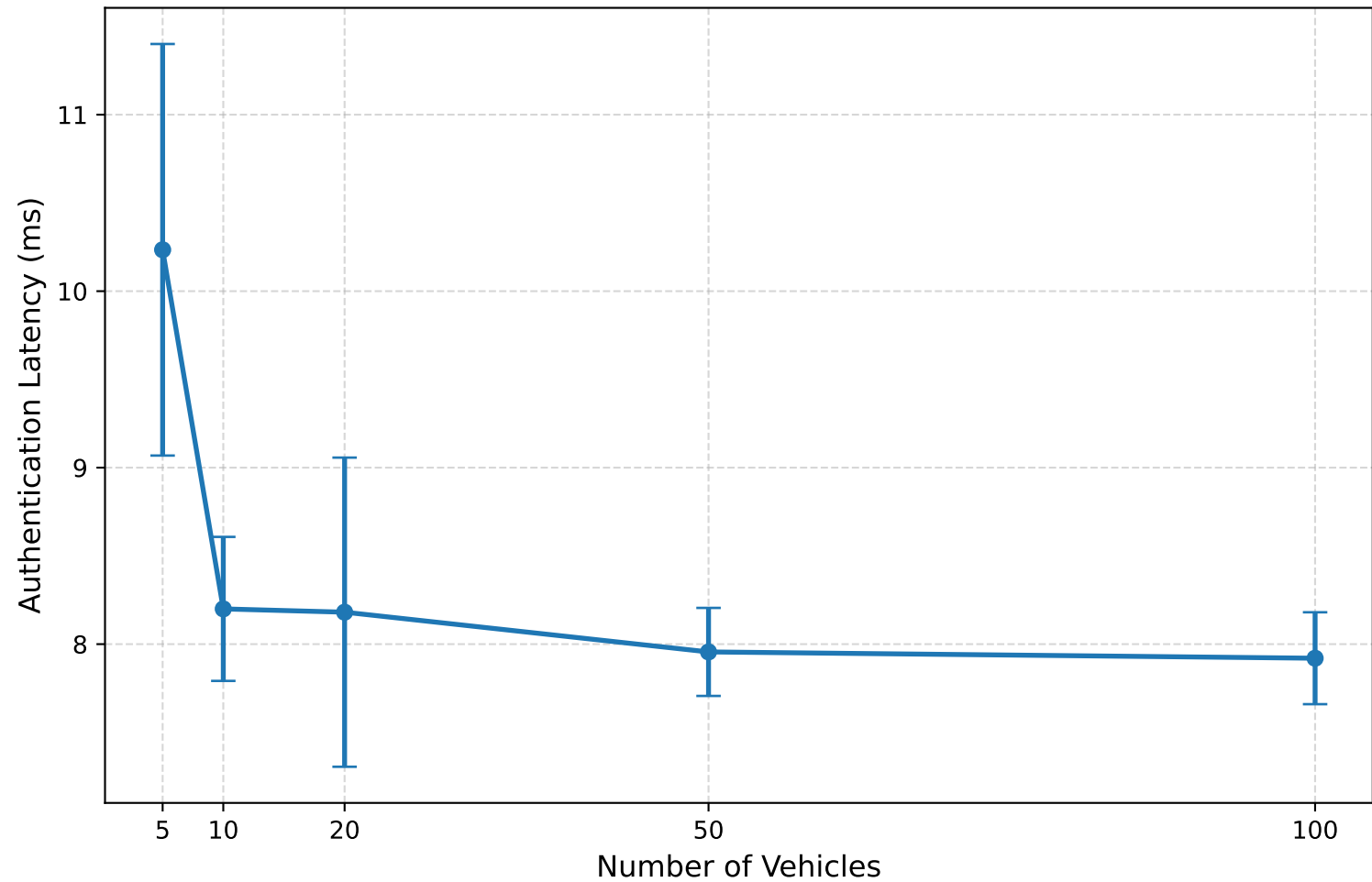
Authentication Latency vs Vehicle Population
