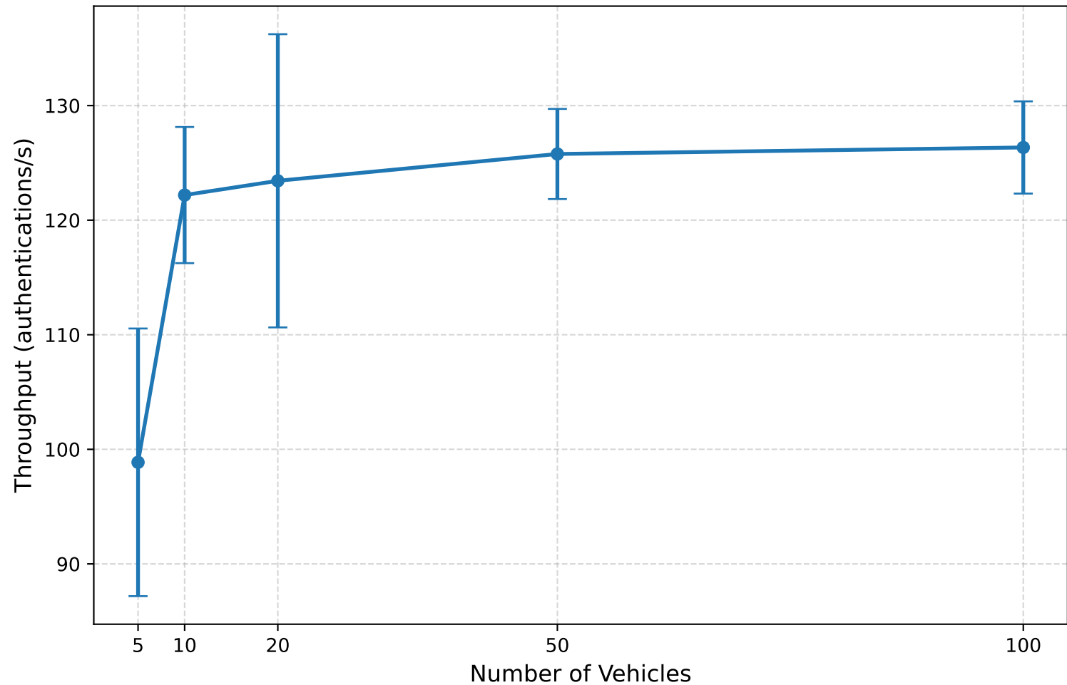
Authentication Throughput vs Vehicle Population
