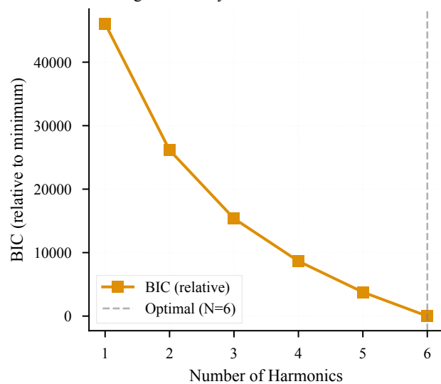
Figure 4D: Bayesian Information Criterion
