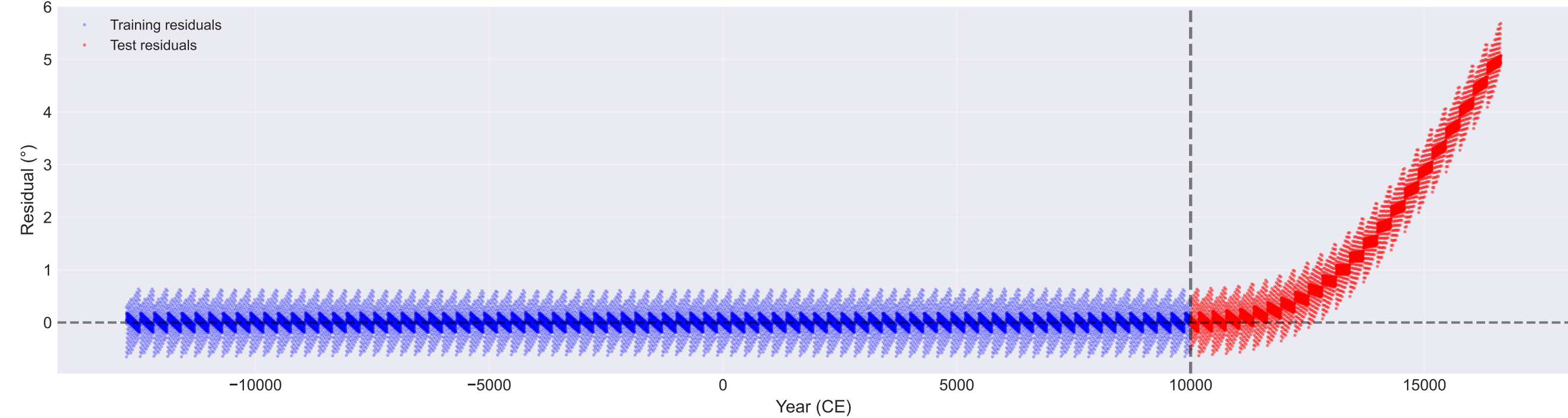
Model Residuals
