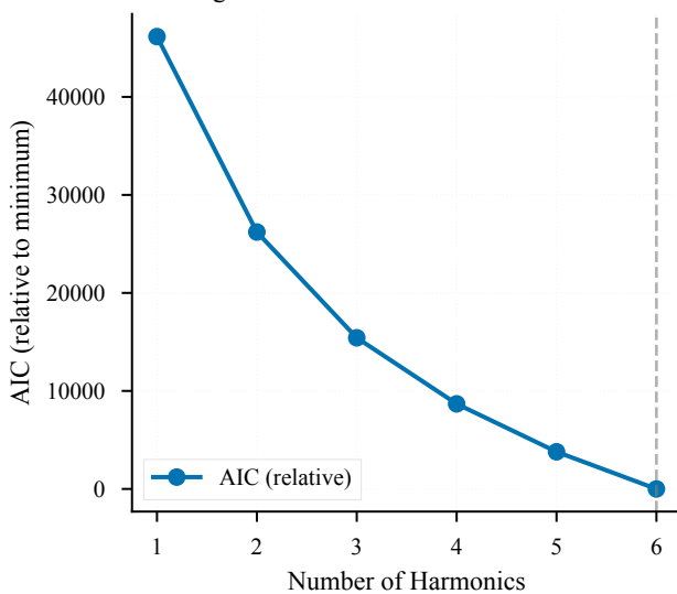
Figure 4C: Akaike Information Criterion
