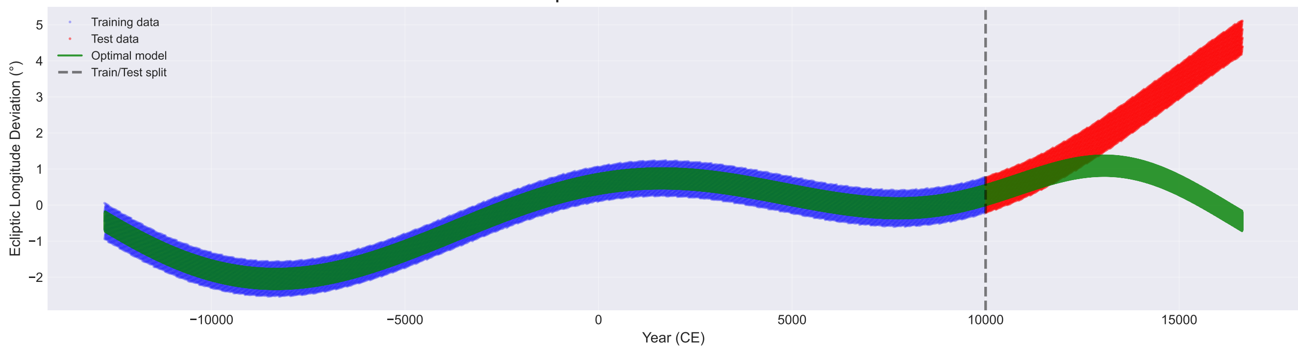
Test Set Performance (RMSE=2.2662°)
