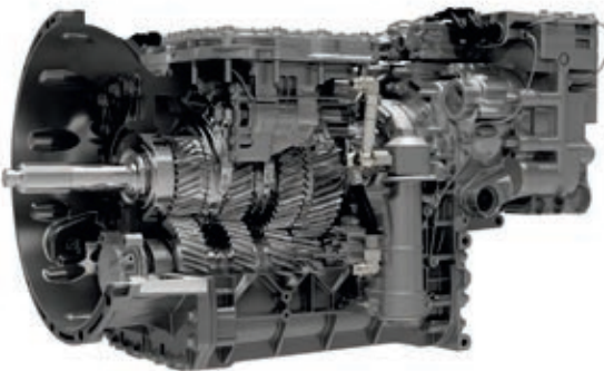
OPTIDRIVER GEARBOX Devoted to challenging applications in 4x4, 6x6 and up to 120 t.
