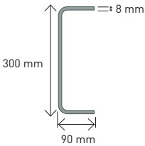
Standard side member
