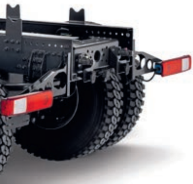
REAR OVERHANG can be customised in 50 mm sections to avoid cutting the side members.
