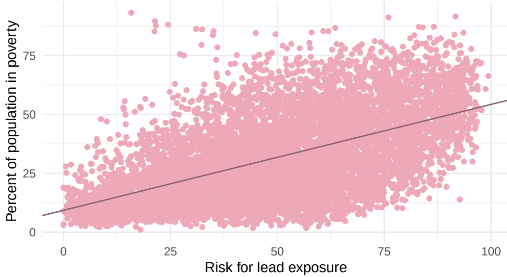
Comparison of lead exposure and poverty for 2010 census tracts in California with fitted simple linear regression model
