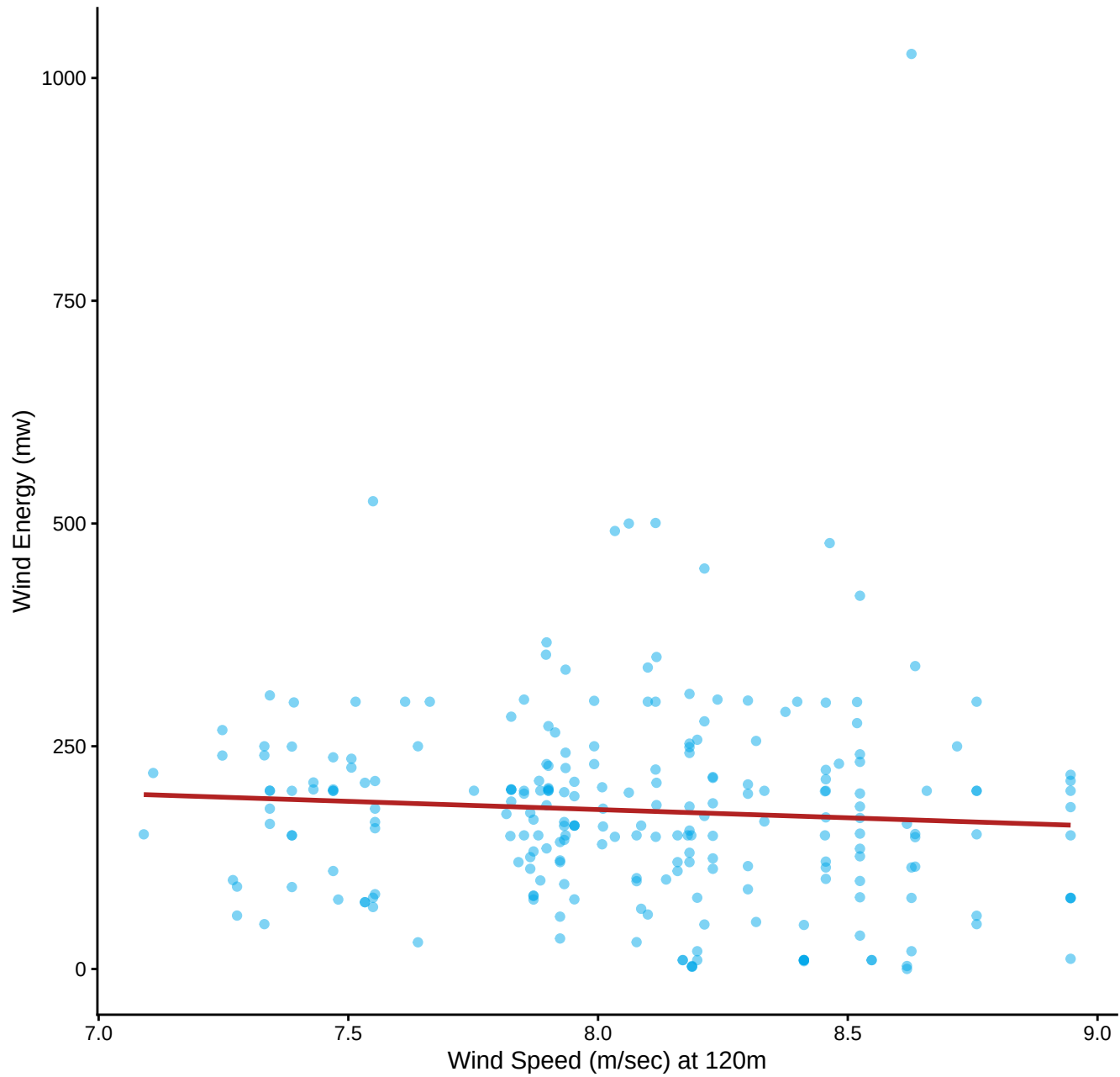
Wind Speeds & Wind Energy Generation
