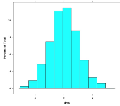
(a) Histogram
