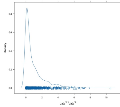
(b) Densityplot
