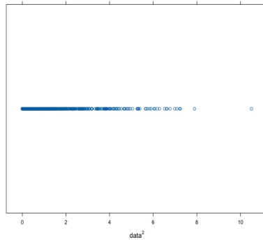
(c) Stripplot
