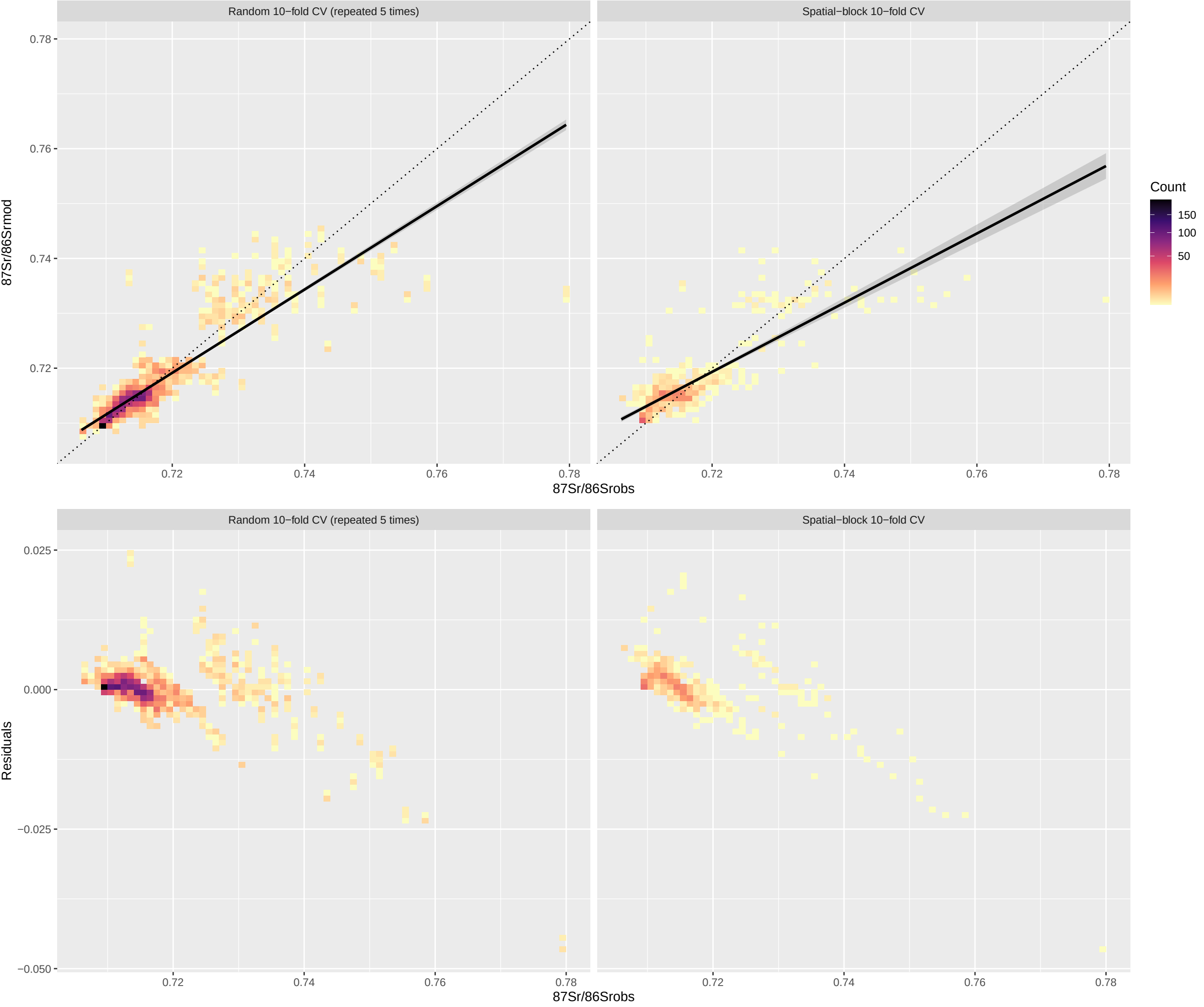
Model performance: random vs. spatial cross-validation
