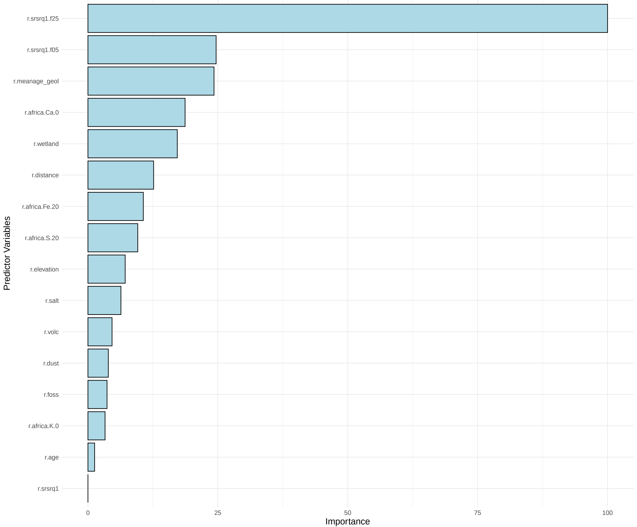
Variable Importance Plot
