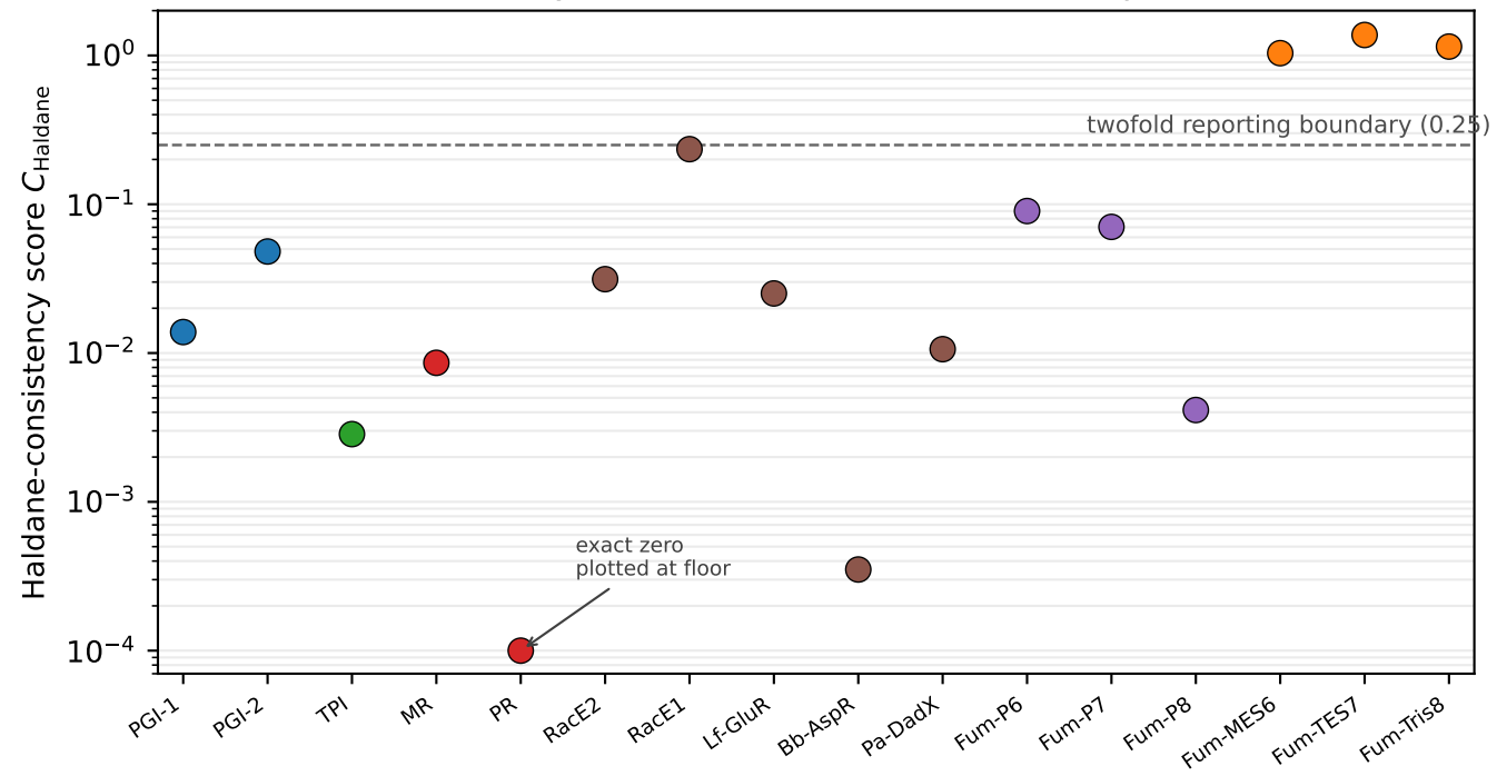
Consistency cost for individual scored comparisons
