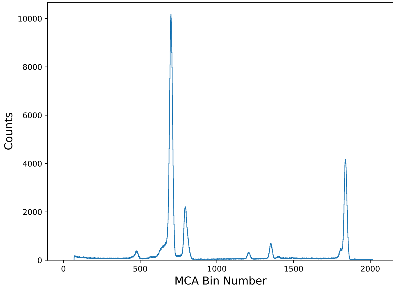
Example ^{133}\text{Ba} Calibration Spectrum
