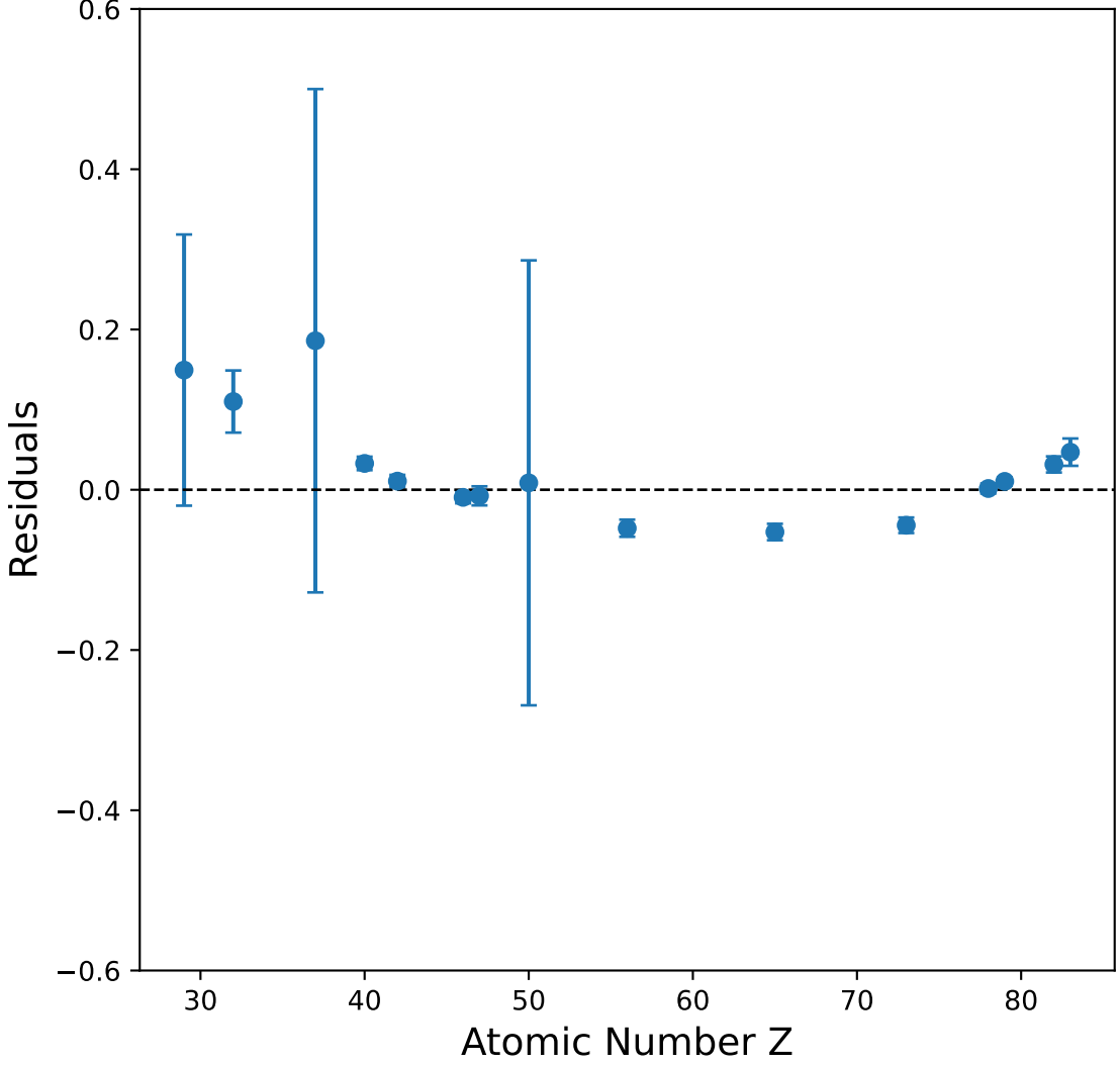
Residuals of Linear Fit to Characteristic K - L_3 X-Ray Energies
