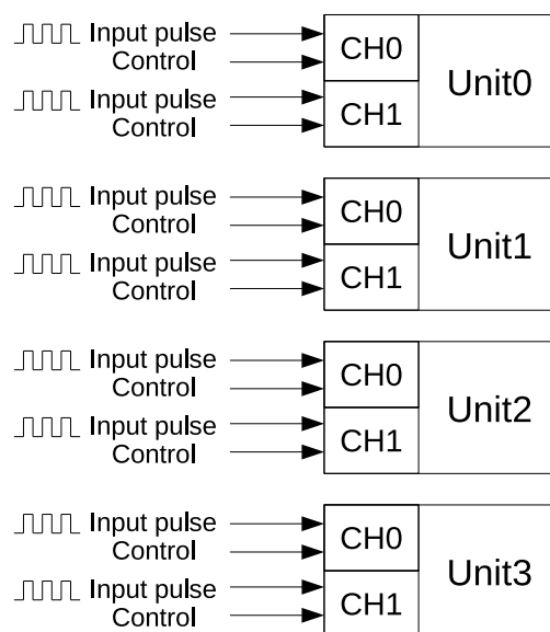
Figure 46.1-1. PCNT Overview
