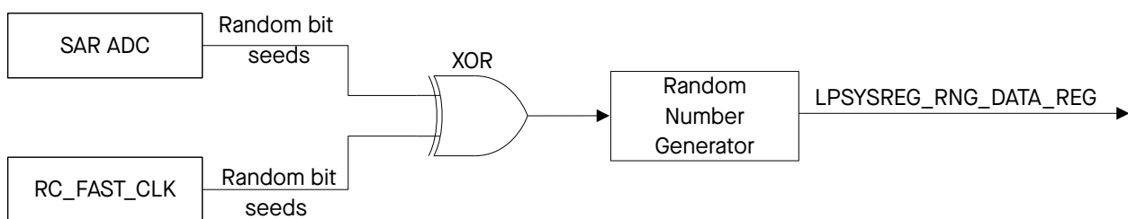
Figure 32.3-1. Noise Source
