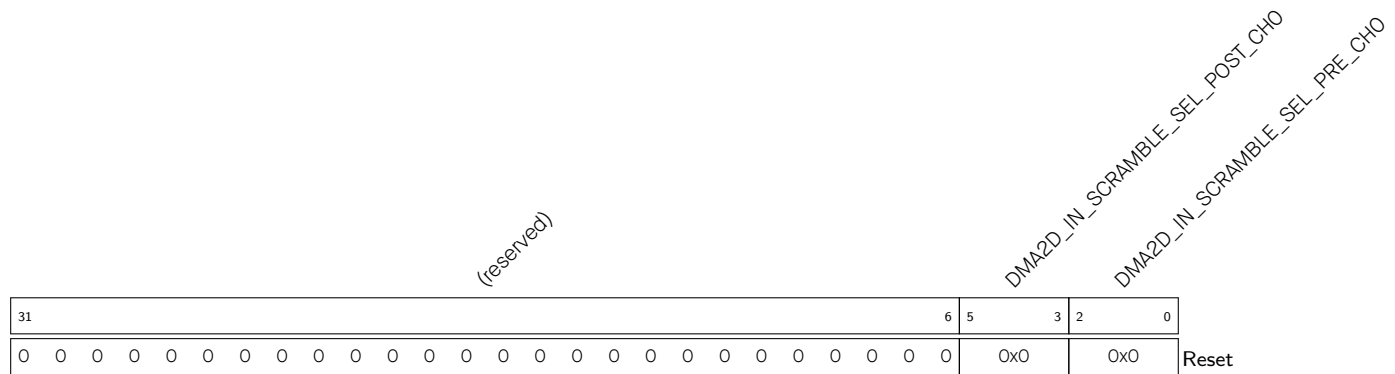
Register 6.24. DMA2D_IN_SCRAMBLE_CHO_REG (0x0550)
