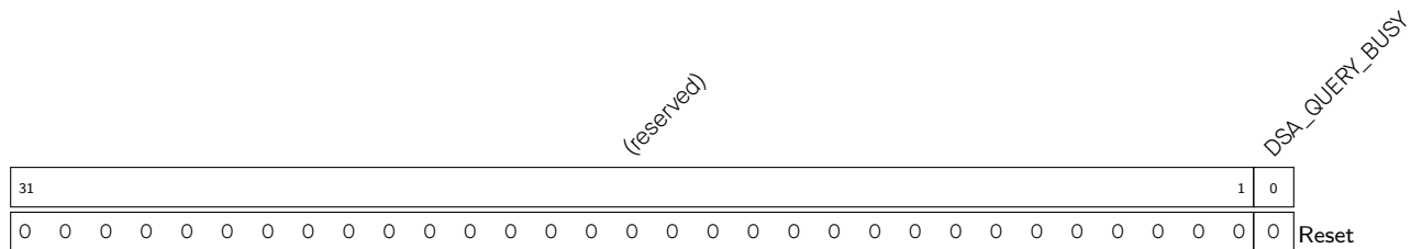
Register 29.5. DSA_QUERY_BUSY_REG (0x0E0C)
