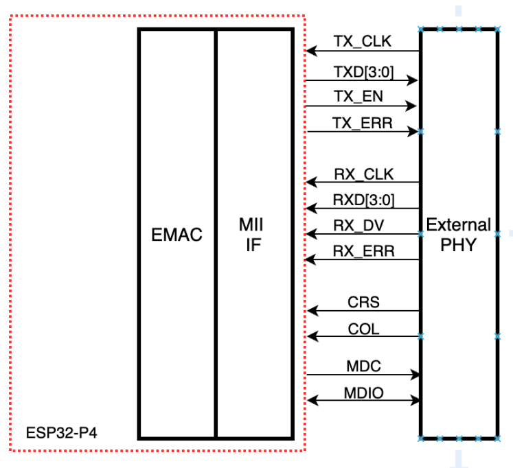
Figure 50.4-3. MII Interface
