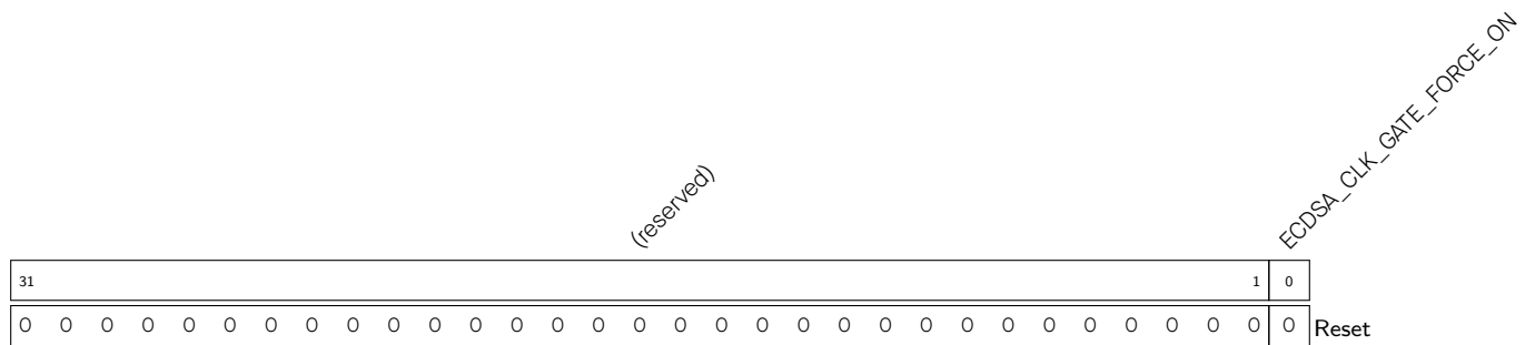
Register 30.3. ECDSA_CLK_REG (0x0008)
