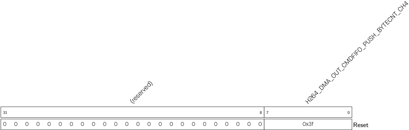
Register 37.224. H264_DMA_OUT_PUSH_BYTECNT_CH4_REG (0x0478)
