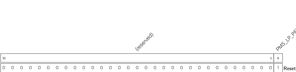
Register 19.76. PMS_LP_PERI_PMS_CLK_EN_REG (0x0004)
