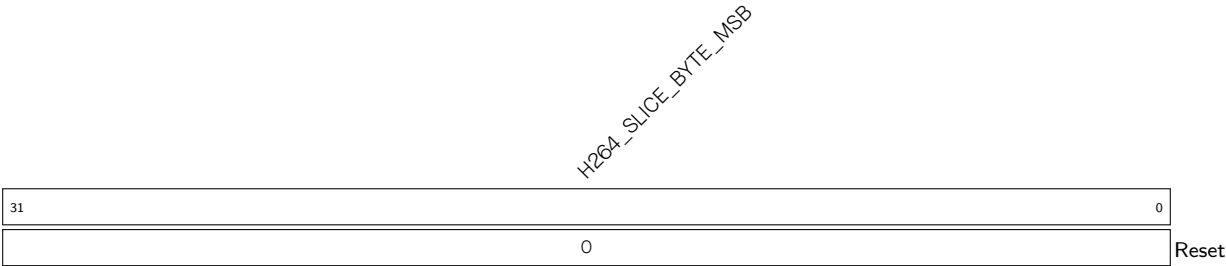
Register 37.45. H264_SLICE_HEADER_BYTE1_REG (0x00BC)
