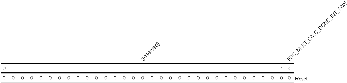
Register 25.1. ECC_MULT_INT_RAW_REG (0x000C)
