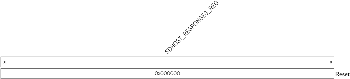
Register 52.32. SDHOST_RESP3_REG (0x003C)
