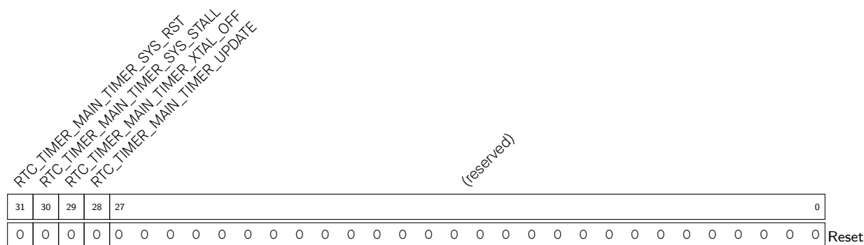
Register 18.5. RTC_TIMER_UPDATE_REG (0x0010)
