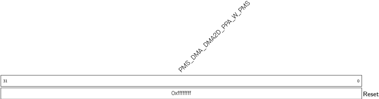
Register 19.52. PMS_DMA_DMA2D_PPA_PMS_W_REG (0x0208)
