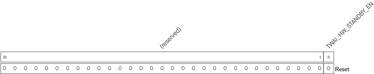
Register 51.8. TWAI_HW_CFG_REG (0x0084)
