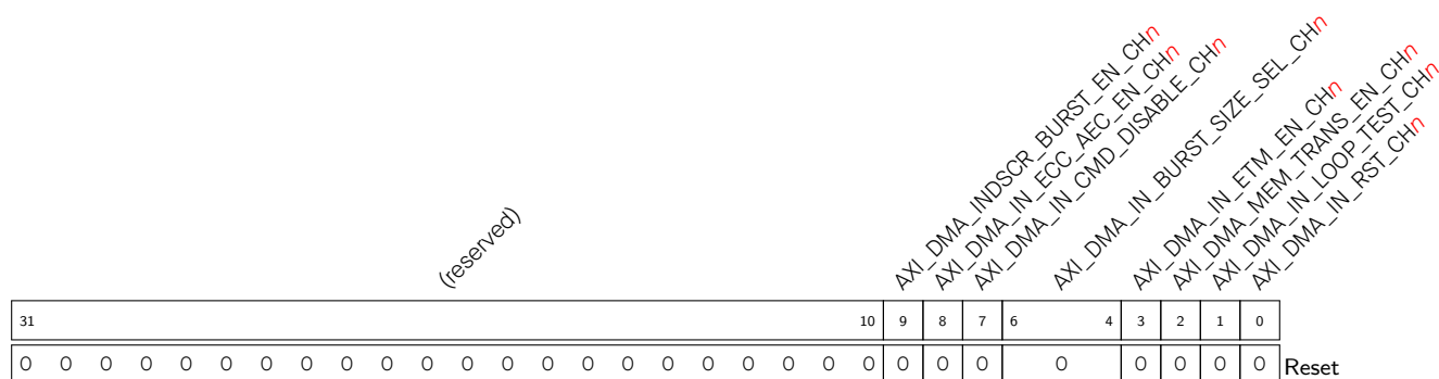
Register 4.74. AXI_DMA_IN_CONFO_CH n _REG ( n : 0-2) (0x0010+0x68* n )
