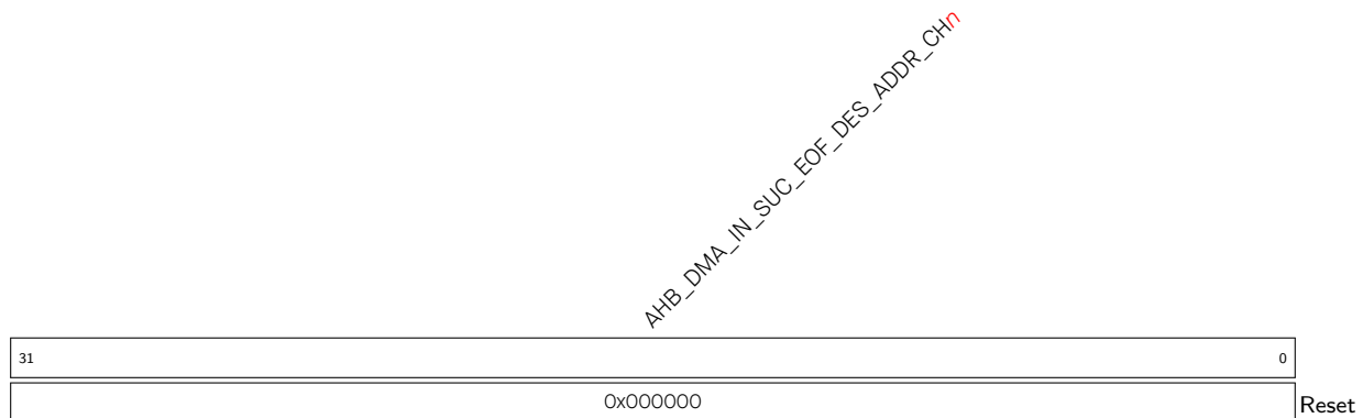
Register 4.50. AHB_DMA_IN_SUC_EOF_DES_ADDR_CH n _REG ( n : 0-2) (0x0088+0xC0* n )
