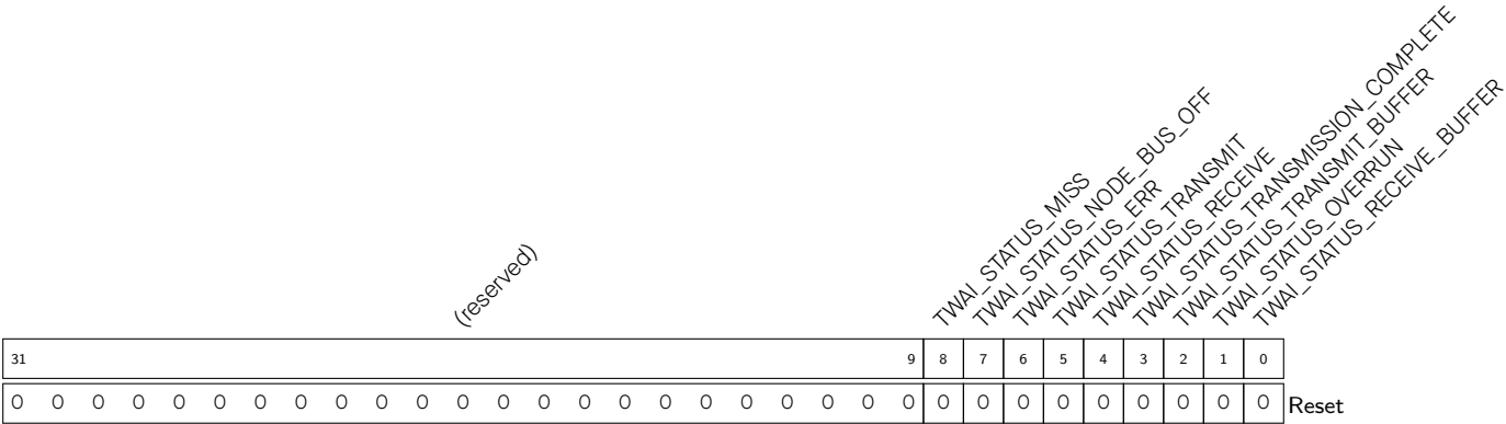
Register 51.11. TWAI_STATUS_REG (0x0008)
