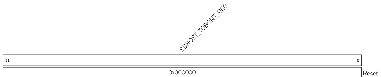
Register 52.36. SDHOST_TCBCNT_REG (0x005C)
