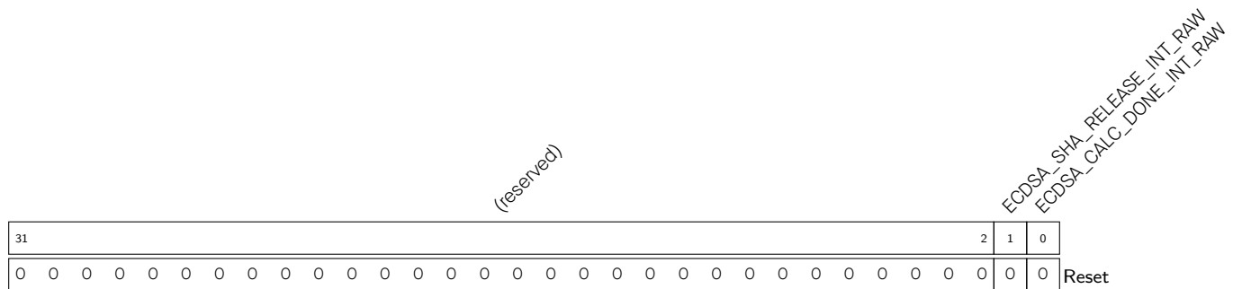
Register 30.4. ECDSA_INT_RAW_REG (0x000C)
