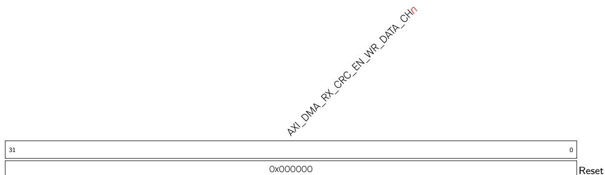
Register 4.127. AXI_DMA_RX_CRC_EN_WR_DATA_CH n _REG ( n : 0-2) (0x0058+0x68* n )
