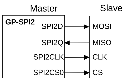
Figure 41.5-6. Full-Duplex Communication Between GP-SPI2 Master and a Slave
