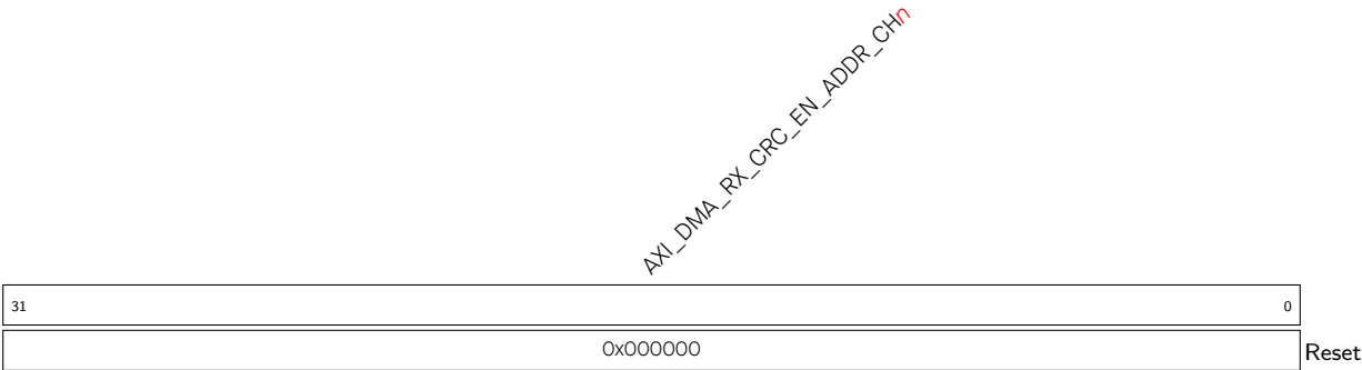
Register 4.83. AXI_DMA_RX_CRC_EN_ADDR_CH n _REG ( n : 0-2) (0x005C+0x68* n )
