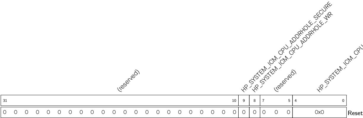
Register 20.78. HP_SYSTEM_ICM_CPU_ADDRHOLE_INFO_REG (0x0044)
