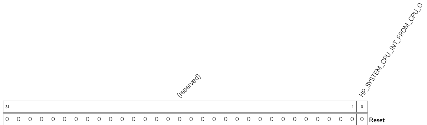
Register 20.3. HP_SYSTEM_HP_CPU_INT_FROM_CPU_0_REG (0x0010)
