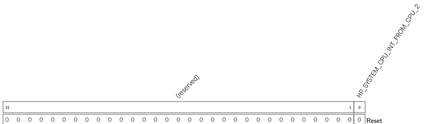
Register 20.5. HP_SYSTEM_HP_CPU_INT_FROM_CPU_2_REG (0x0018)
