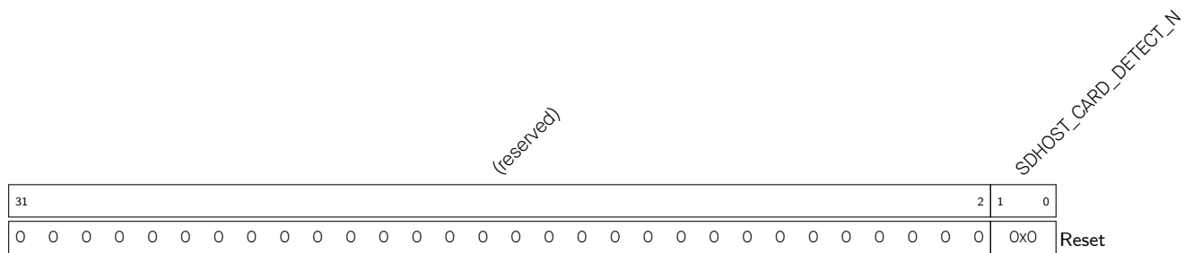
Register 52.34. SDHOST_CDETECT_REG (0x0050)
