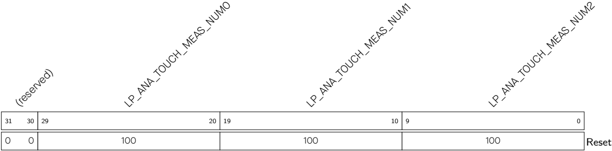
Register 58.16. LP_ANA_TOUCH_WORK_MEAS_NUM_REG (0x010C)
