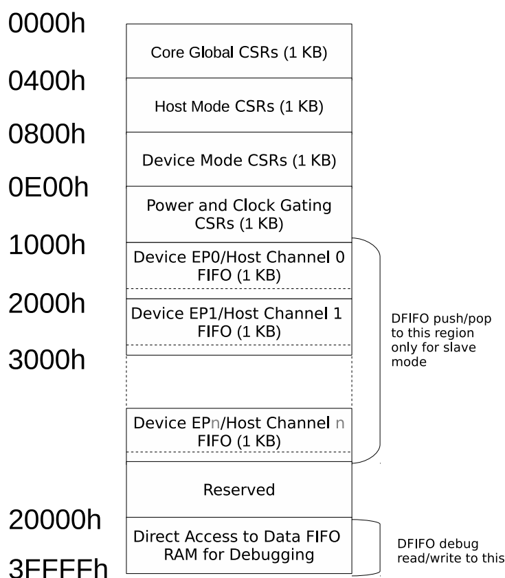
Figure 48.4-2. OTG_FS Register Layout
