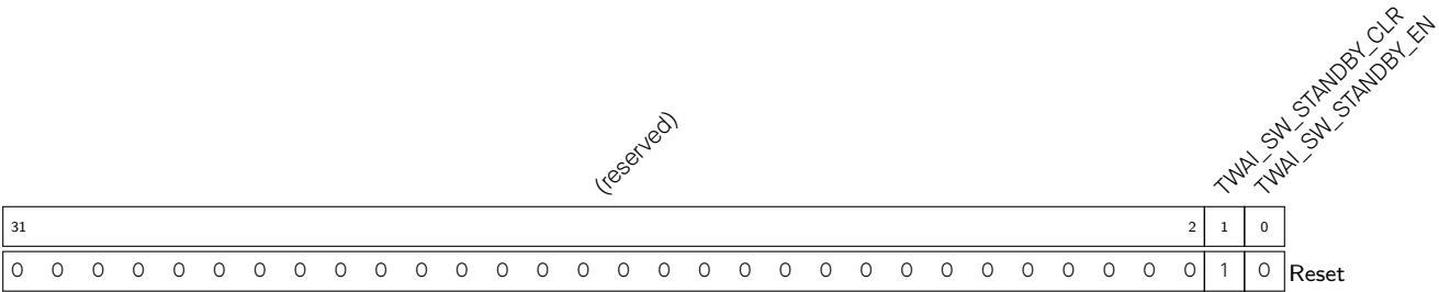
Register 51.7. TWAI_SW_STANDBY_CFG_REG (0x0080)
