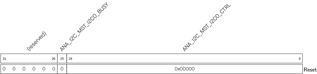
Register 43.1. ANA_I2C_MST_I2CO_CTRL_REG (0x0000)
