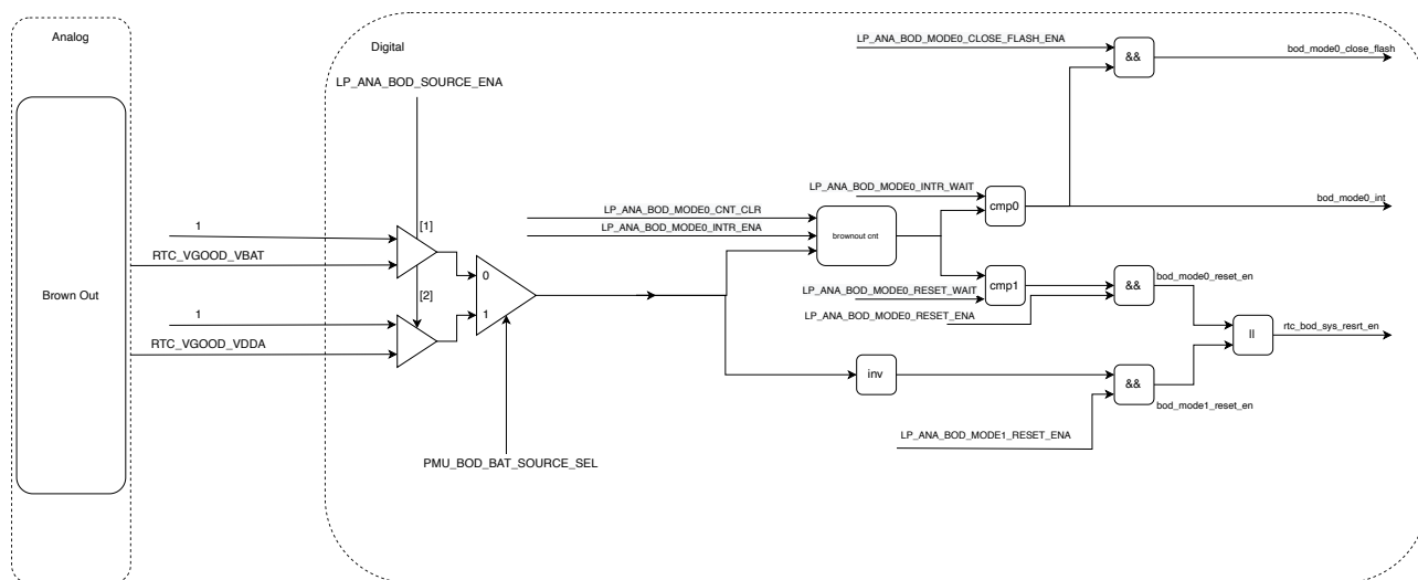
Figure 23.3-1. Brown-out Detector Overview
