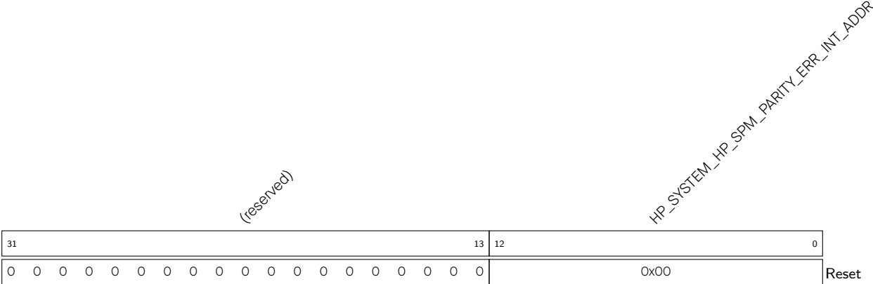
Register 20.40. HP_SYSTEM_HP_SPM_PARITY_ERR_RECORD_REG (0x010C)
