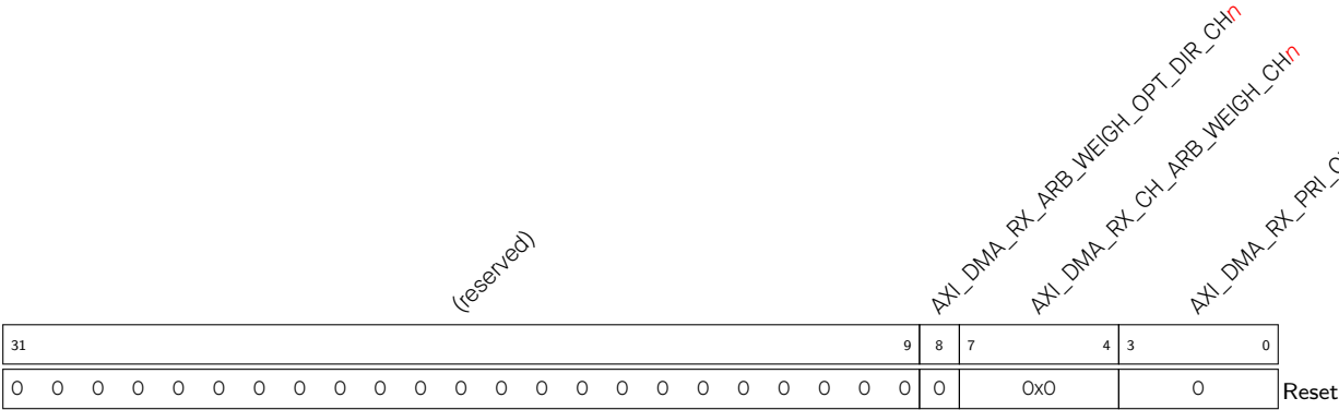
Register 4.123. AXI_DMA_IN_PRI_CHn_REG (n: 0-2) (0x0040+0x68*n)
