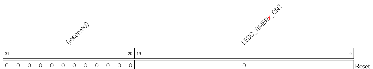
Register 53.13. LEDC_TIMER x _VALUE_REG (x: 0-3) (0x00A4+0x8*x)
