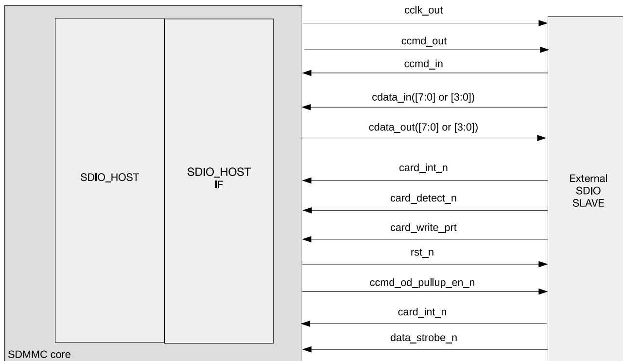
Figure 52.3-1. SD/MMC Controller External Interface Signals
