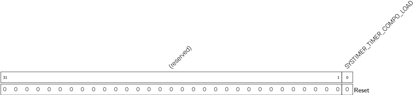
Register 15.17. SYSTIMER_COMPO_LOAD_REG (0x0050)
