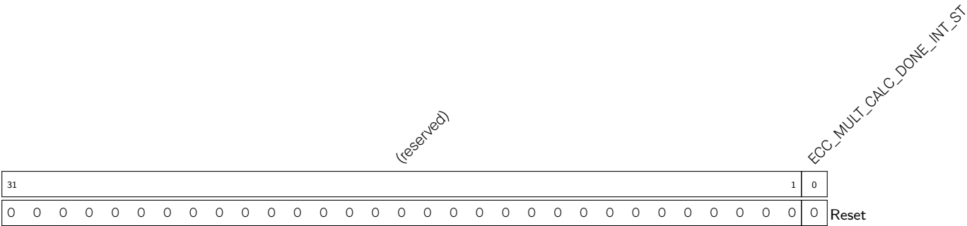
Register 25.2. ECC_MULT_INT_ST_REG (0x0010)
