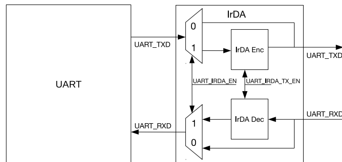
Figure 40.4-7. IrDA Encoding and Decoding Diagram
