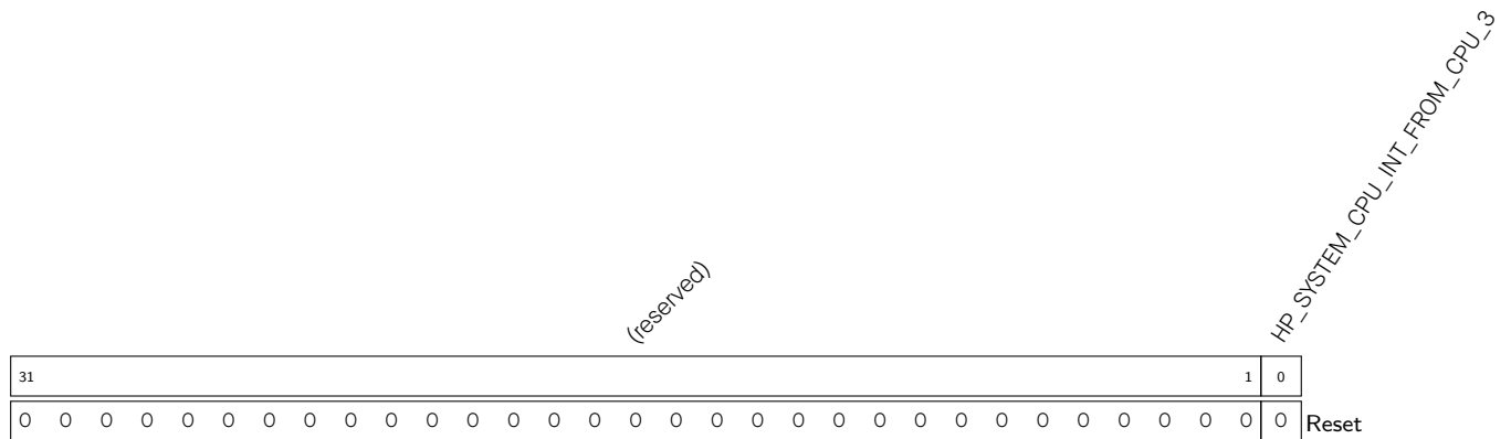
Register 20.6. HP_SYSTEM_HP_CPU_INT_FROM_CPU_3_REG (0x001C)
