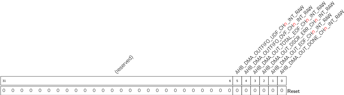
Register 4.5. AHB_DMA_OUT_INT_RAW_CHn_REG (n: 0-2) (0x0030+0x10*n)
