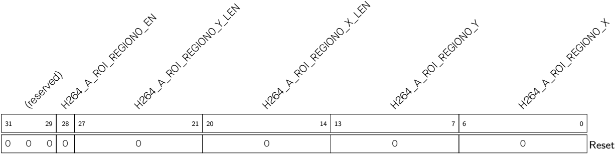
Register 37.10. H264_A_ROI_REGIONO_REG (0x0024)
