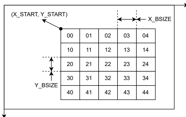
Figure 34.5-2. Sub-Window Numbering
