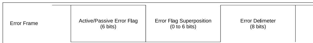
Figure 51.2-2. Fields of an Error Frame
