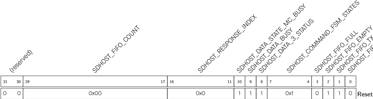
Register 52.33. SDHOST_STATUS_REG (0x0048)
