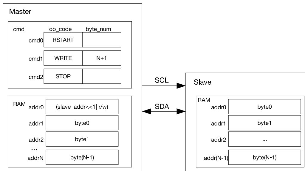
Figure 42.6-1. I2C master Writing to I2C slave with a 7-bit Address
