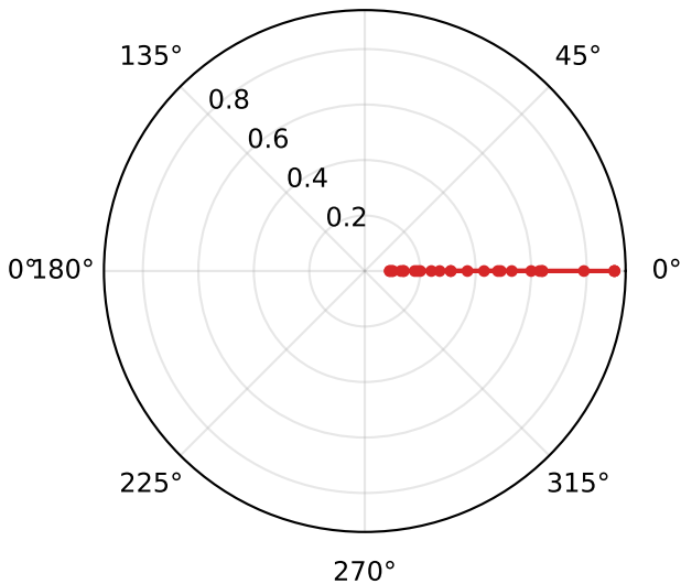
left arm right arm Continuous reachability from home, median of 10 sweeps (m)
