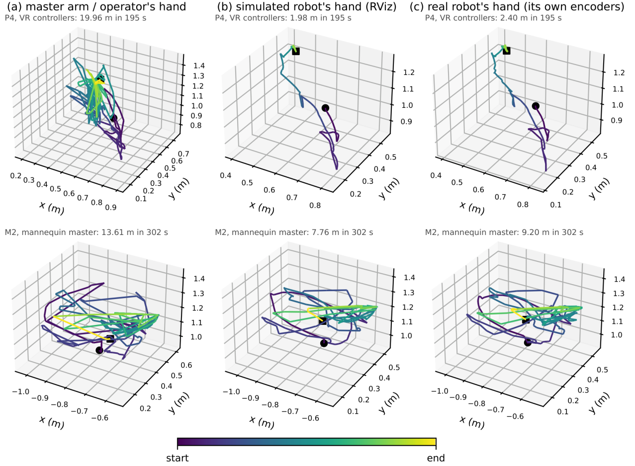
Figure 3.10: One session per cohort as three separate paths, coloured from start to end: (a) the master arm or operator's hand, (b) the simulated robot's hand as RViz shows it, (c) the real robot's hand from its own joint encoders. Top: VR (P4, object tracking, direct; simulated-to-real gap 11.1 mm). Bottom: mannequin master (M2, target reaching, direct; gap 21.8 mm). The hand covers far more distance than the robot because the mapping scales and filters it. Every session: Chapter O .
