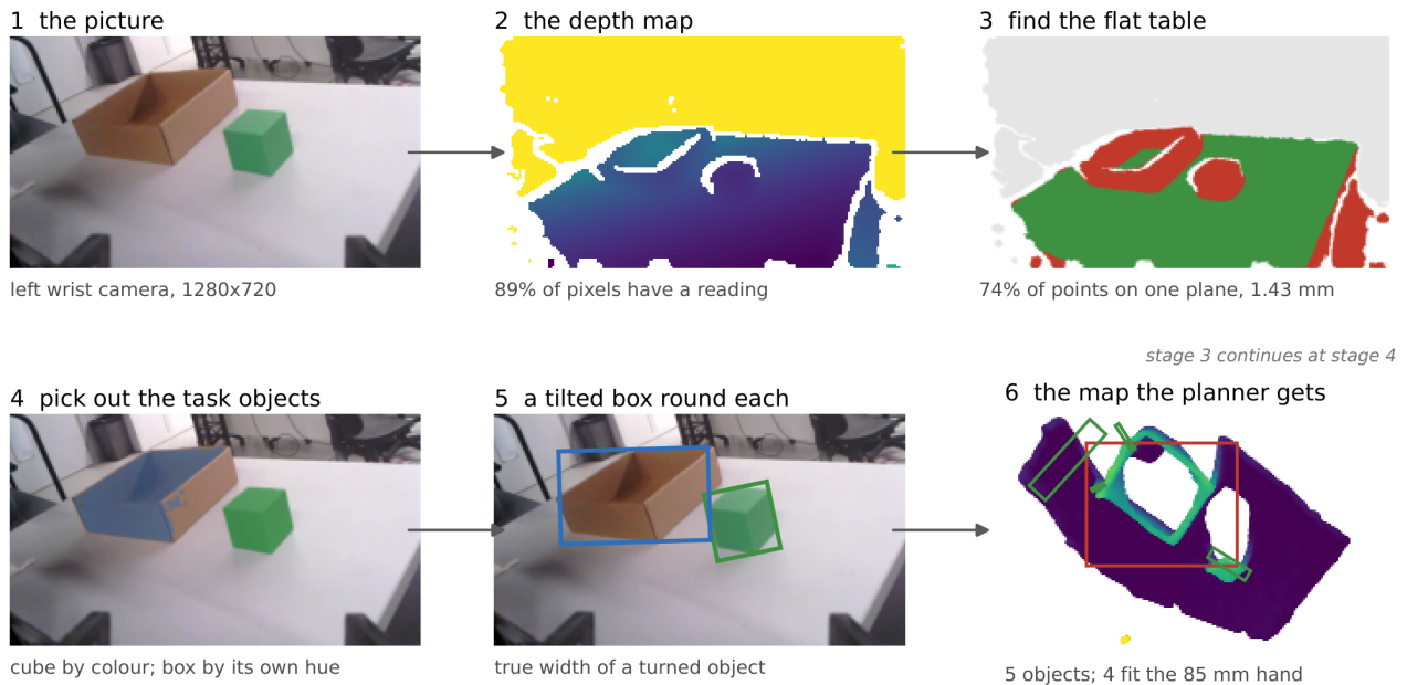
Figure 3.3: The pipeline on one real left-wrist-camera frame, stage by stage: picture; depth map; table plane (74 % of points on it, 1.43 mm); the two task objects picked out; a tilted box round each; and the map handed to the planner – five objects, four fit the 85 mm hand, the widest is 341 mm.
