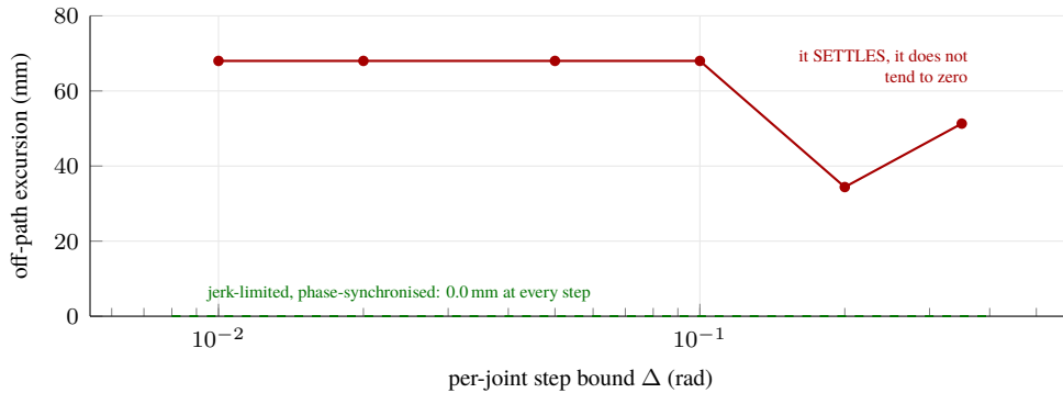
Figure 10.1: The excursion is a property of the algorithm, not of its tuning. Sweeping the per-joint step bound over a factor of 35 does not drive the excursion toward zero: it settles at 68 mm, and is in fact worse at small steps than at the shipped one. Section 8.1.3 gives the reason — the clamped step is parallel to the required displacement only when every joint is inside the bound or every joint is saturated equally, and at no step size is that generally true. Each point is a genuinely different path densified at 0.02 rad, not one path sampled at different rates.
