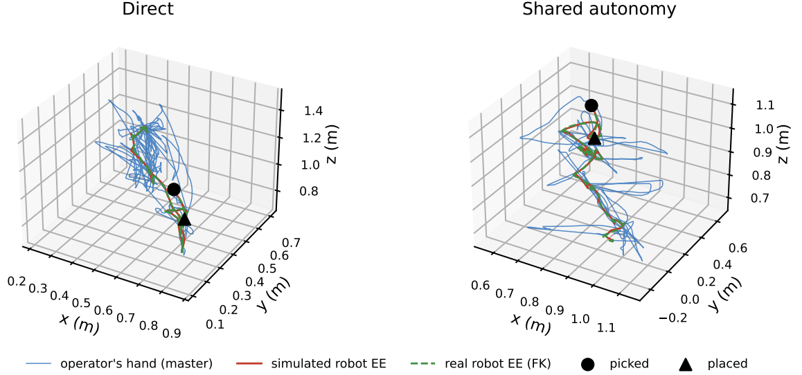
Figure 4.5: Master hand, simulated robot end-effector, and the real robot’s own end-effector (forward kinematics on its own encoders, not simulated) – one Direct and one Shared-autonomy session, same operator and task, with picked and placed marked from the gripper’s own logged transitions. Simulated and real agree closely throughout, the same small gap as Fig. 4.6; master moves far more, since the mapping scales and filters it.
