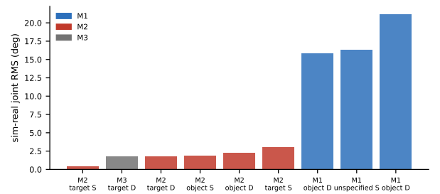
(b) master-arm cohort, every session
