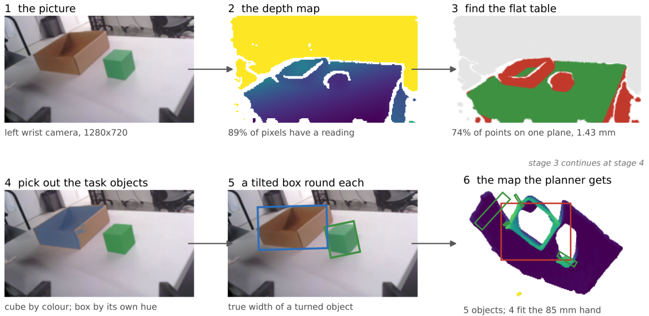
Figure 3.3: The pipeline on one real left-wrist-camera frame, stage by stage: picture; depth map; table plane; the two task objects picked out; a tilted box round each; and the map handed to the planner – five objects, four fit the 85 mm hand, the widest is 341 mm.
