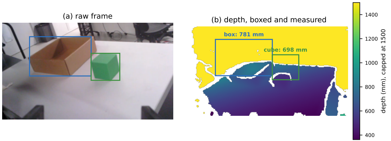
Figure 3.4: Figure 3.3’s frame (a) beside its depth map (b), each object boxed and labelled with its median measured distance.
