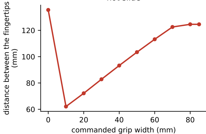
(b) the fingers swing, they do not slide
