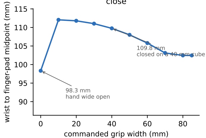
(a) the pads move as the fingers close
