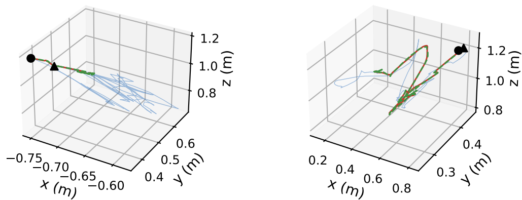
P1, pick and place, direct control (gap 14 mm) and place, with assistance (gap 11 mm)
