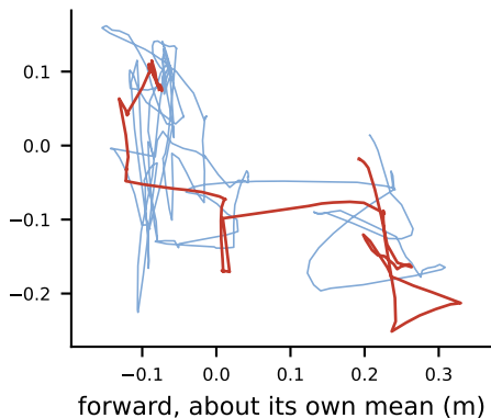
P5, pick and place, direct control
