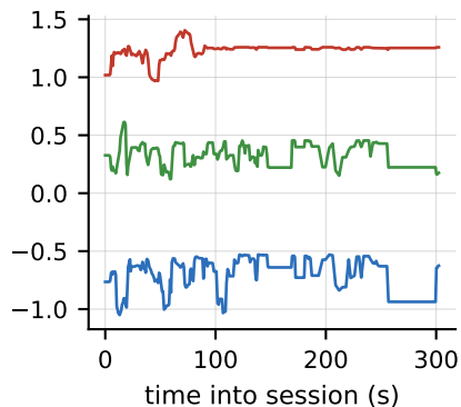
mannequin master position (m)
