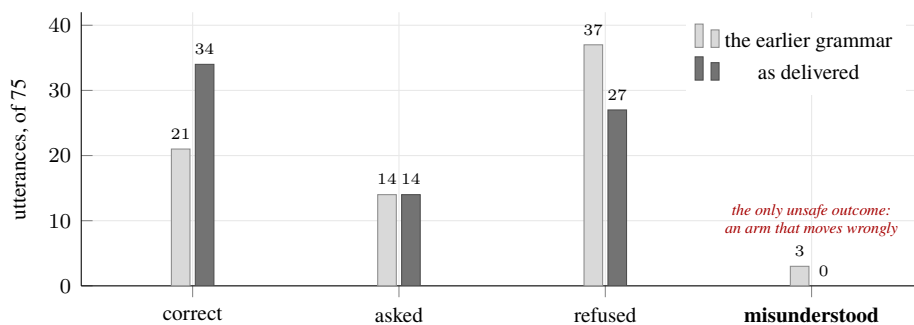
Figure 10.3: Seventy-five phrasings of one task — selectors, compounds, bare picks, politeness and misspellings — scored against the delivered grammar and against the grammar as committed at an earlier revision, checked out of version control and run in its own interpreter, so the two columns differ by the code and by nothing else. Asked and refused are safe outcomes: the arm does not move and the operator is told why. Misunderstood is the only unsafe one, because it is the outcome in which the arm moves and does the wrong thing.
