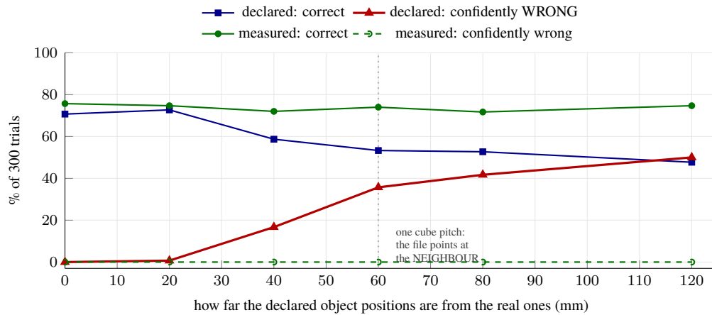
Figure 10.2: Intent inference over 300 trials per point, four candidate objects on a 60 mm pitch. The quantity that matters is not the correct rate but the confidently wrong rate, because a wrong answer held with confidence is the one state in which this system assists an operator toward an object they were not reaching for. Working from declared coordinates, it reaches 50 % once the declaration is one cube pitch out. Working from measured ones it stays at 0.0 % across the whole sweep, and the correct rate stays flat at 71.7 to 75.7 %.
