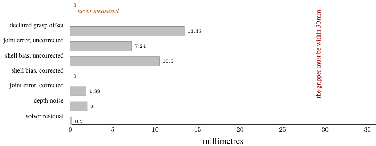
Figure 7.1: Contributions to positioning error at closure, each measured separately by scripts/measure_control_budget.py . Terms marked corrected are available and switched off. Combined in quadrature the measured terms give 18.6 mm; added, as systematic terms may be, they give 33.4 mm against a 30 mm requirement. The orange bar is the transform between the camera frame in the robot description and the physical camera module, which has never been measured and is now the largest unknown in the budget.
