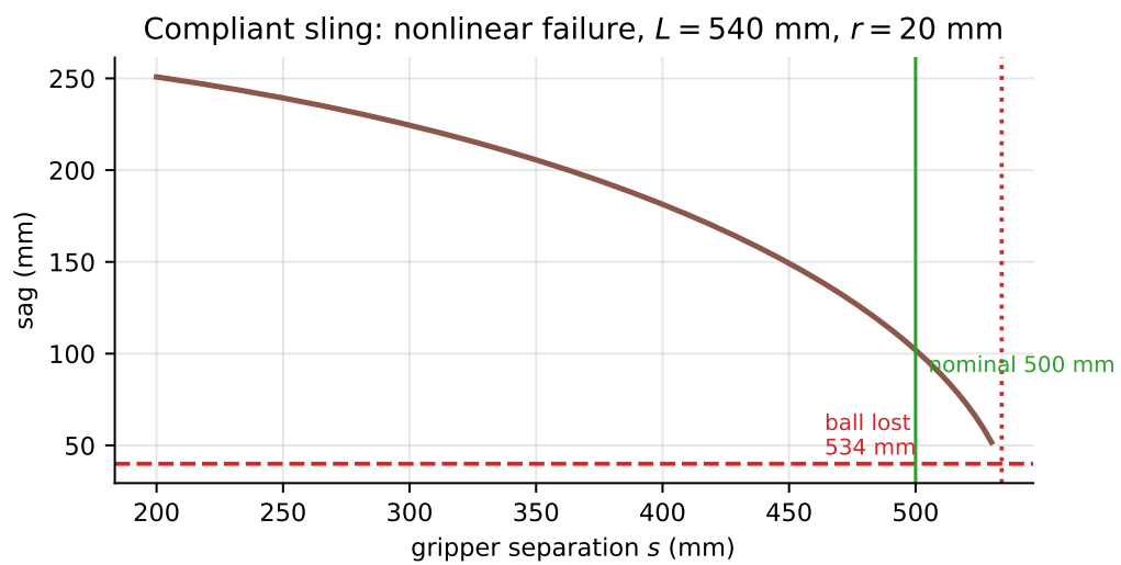
Figure 10.7: Sag against gripper separation for the re-specified compliant carrier. The nonlinearity is the point: sag falls slowly, then the ball is lost abruptly at 534 mm.
