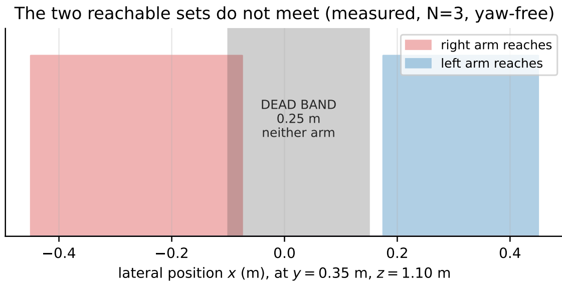
Figure 10.3: The two reachable sets do not meet. Measured at y = 0.35 m, z = 1.10 m with yaw free and three repeats per point.
