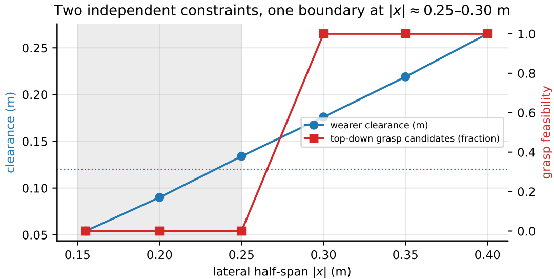
Figure 10.5: Wearer clearance and top-down grasp feasibility against lateral half-span. The two constraints were measured independently and for different purposes, and both place the usable boundary at |x| \approx 0.25 to 0.30 m.
