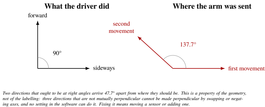
Figure 9.3: Two master motions intended to be orthogonal arrive 137.7^\circ apart at the commanded end effector. The test is independent of any axis labelling, which is what makes this a geometric limitation rather than a calibration error.
