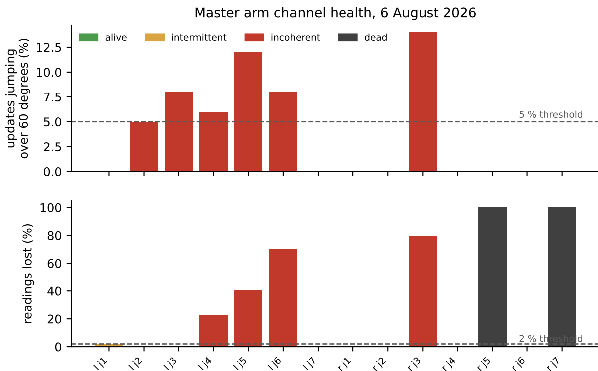
Figure 9.1: Every channel on both quantities that decide its verdict, with the thresholds marked and the verdict carried in the bar colour. The upper panel is the discriminating one: a channel above the five per cent line is returning values that are present, fresh and not a trajectory. Regenerated from recordings/baselines/channels_20260806.json by figures/make_figures.py .
