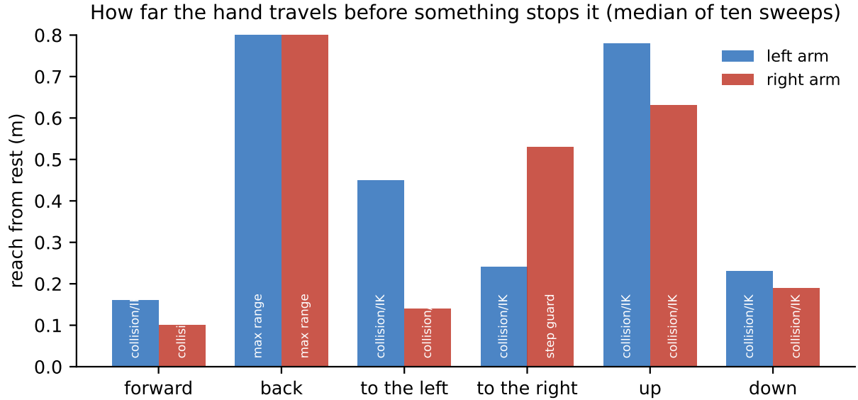
Figure J.1: Continuous reachability from the home pose in the six principal directions, median of ten sweeps, with the binding constraint printed inside each bar. The envelope is markedly anisotropic: the median reach over all twenty-six directions is 0.34 to 0.40 m while the worst direction is 0.14 m on the left arm and 0.09 m on the right. Max range marks a direction in which the sweep exhausted its own travel before the arm did, so those two figures are lower bounds. Regenerated from recordings/baselines/workspace_n10_20260806.json .
