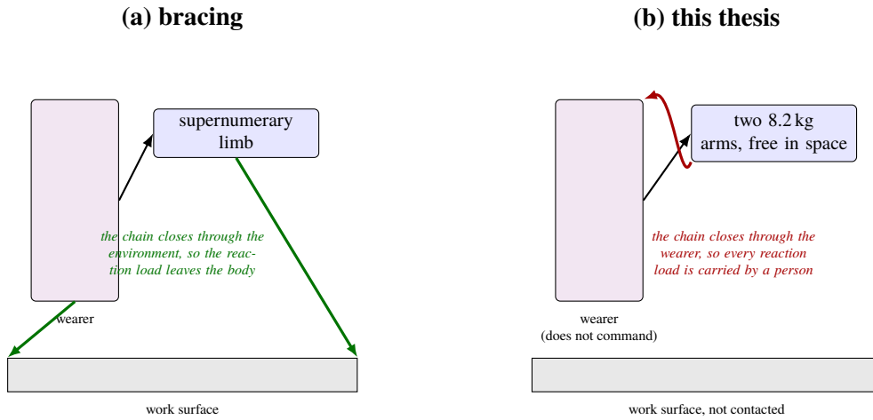
Figure A.1: Two load paths, drawn from the mechanical argument rather than reproduced. In the bracing configuration that established the field [26] the limb anchors against the work surface, so the kinematic chain closes through the environment and the reaction load leaves the body. In the arrangement studied here the arms are free in space, so the chain closes through the wearer and every reaction load is carried by a person who is not the person commanding the motion. This difference, and not the control law, is what makes the wearer’s clearance the binding constraint of Chapter J .
