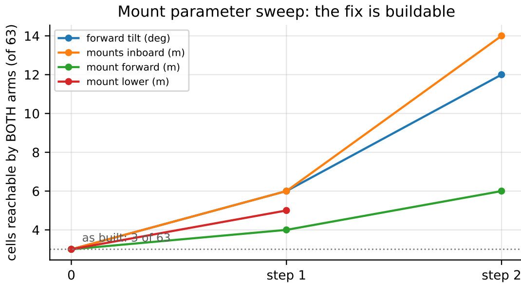
Figure J.4: Single-parameter sweeps from the as-built mount. Forward tilt and inboard translation both help substantially; splaying the mounts outward hurts . The sweep is purely kinematic, moving the arms’ bases without moving the wearer, so these are upper bounds and any candidate requires a clearance check before adoption.
