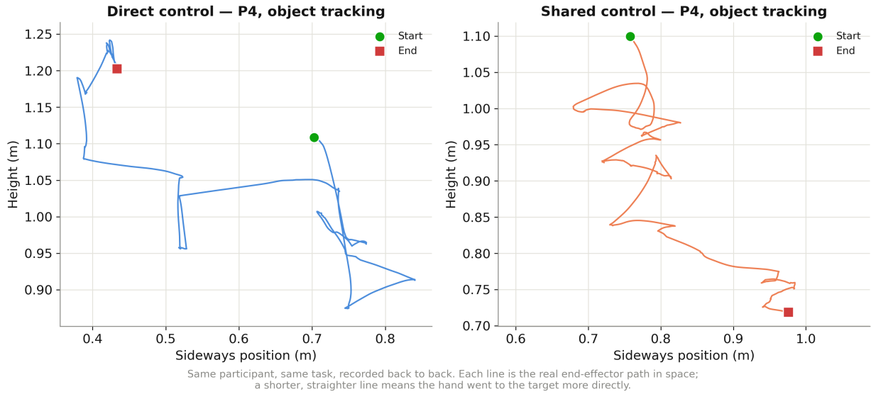
Figure T.6: The actual recorded end-effector path in space for one participant on the same task under both conditions, recorded back to back. Neither path is smooth; a shorter, straighter line would indicate a more direct approach to the target.
