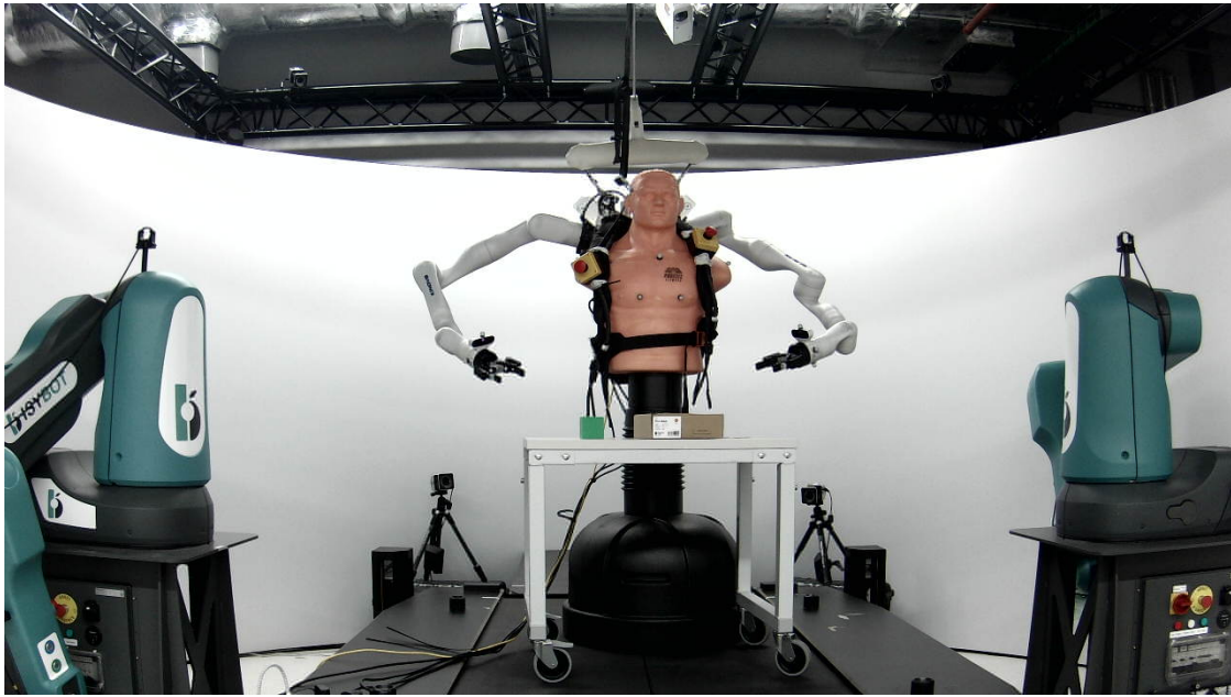
Figure A.3: The platform as built, photographed by the scene camera during the vision session of 2026-08-30. Two Kinova Gen3 arms are carried on a backpack frame on a torso mannequin; the wearer's own arms are absent from this photograph because the frame is instrumented rather than worn during a bench session. The two teal columns are the laboratory's fixed manipulators and are not part of this system. This is a 1280 \times 720 frame from the uncalibrated HD webcam of Chapter E , reproduced here because it is the only view that shows the mount, the arms and the work surface in one frame at the geometry every measurement in this thesis was taken at.
