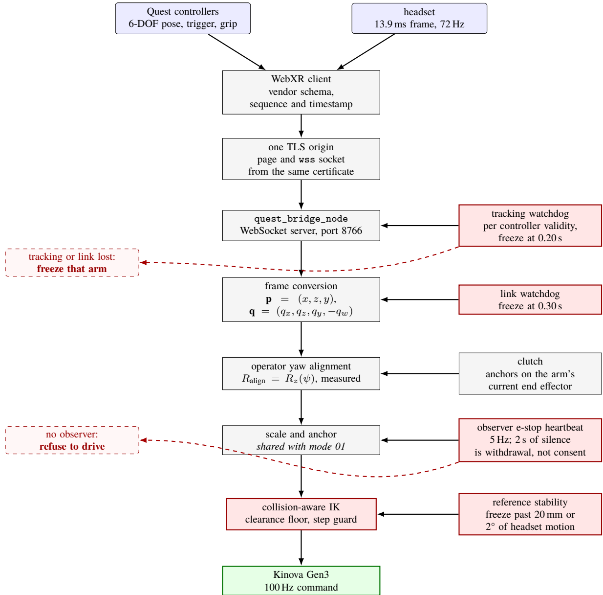
Figure D.5: Mode 02, direct teleoperation from a Quest headset. The headset supplies six degrees of freedom directly, so neither the spherical decomposition nor the channel-health layer of Fig. D.4 appears; everything from scale and anchor downwards is the same code. Four guards are specific to this path, and three of the four were added after a measurement showed the fault they cover was undetectable (Section D.4.2).
