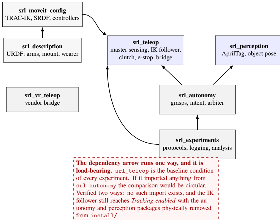
Figure D.1: Package decomposition and the one-way dependency graph.
