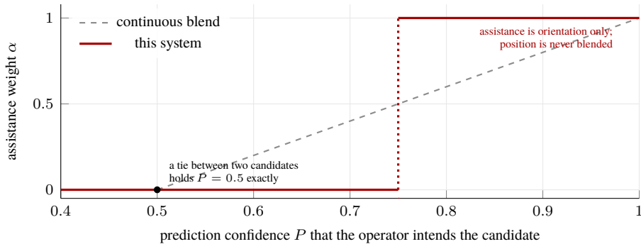
Figure A.2: Arbitration as a function of prediction confidence, plotted from this system’s own constants. Policy blending in its original form [7] raises the assistance weight \alpha continuously with confidence, which means that at low confidence the arm is already moving somewhere the operator did not ask for. The rule implemented here is a threshold: below \theta the assistance weight is exactly zero, and a tie between two adjacent candidates holds P = 0.5 and is therefore never assisted. The distinction matters on this platform because the cost of assisting toward the wrong candidate is not a slower trial but a manipulator moving toward a person who did not command it.
