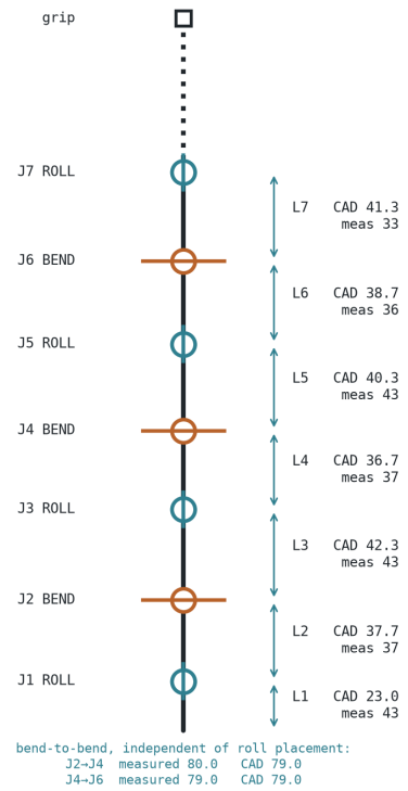
(c) Link lengths inferred from the model against the lengths measured on the built arm.
