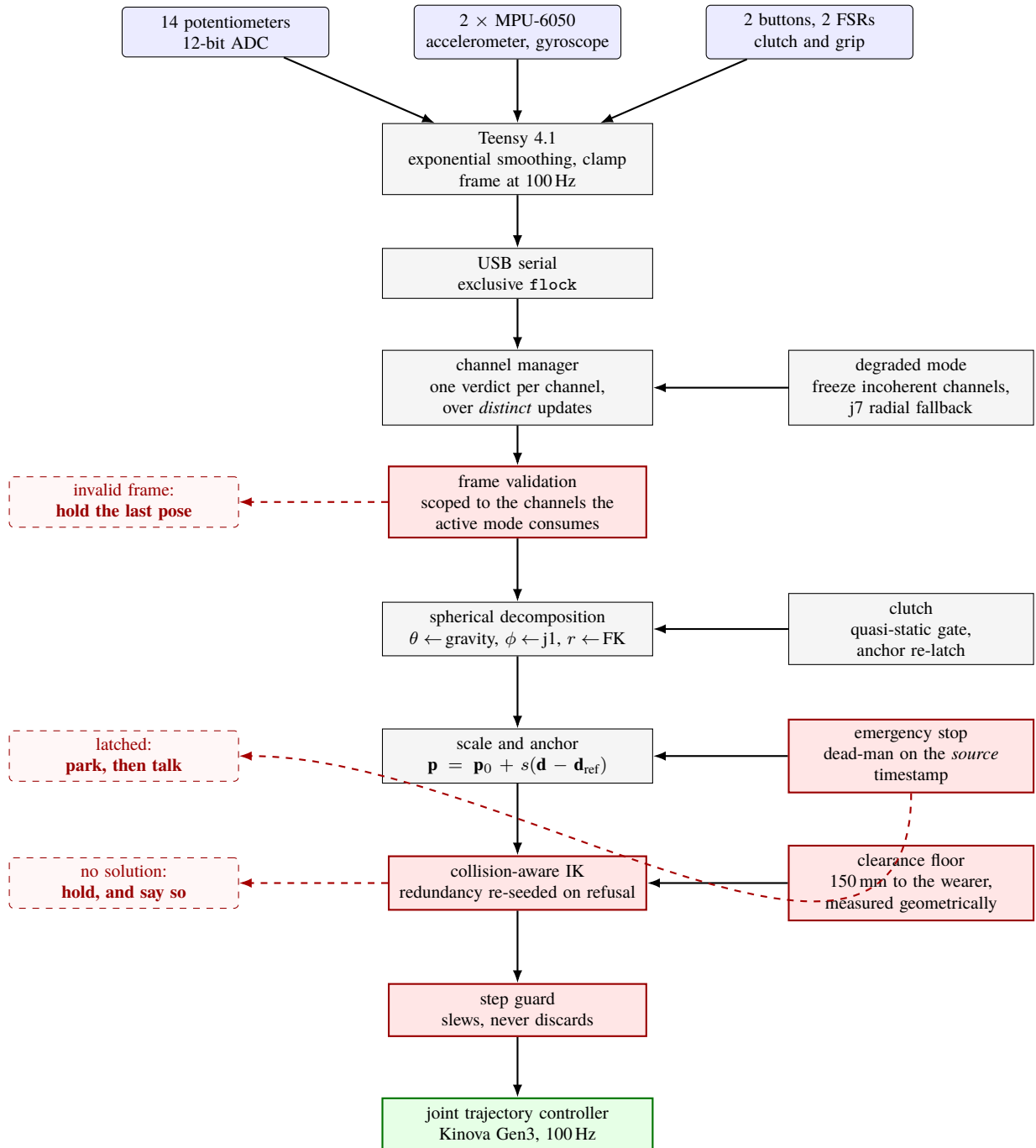
Figure D.4: Mode 01, direct teleoperation from the mannequin master. The centre column is the command spine; guards and side inputs enter from the right; a dashed red arrow leaves to the left for each way a stage can refuse, and names what the arm does instead. Blue is sensing, grey is processing, red is a stage that can stop the arm, and green commands motion. The same three-column grid is used for Figs. D.5 to D.7, so the four paths can be read against one another stage by stage.
