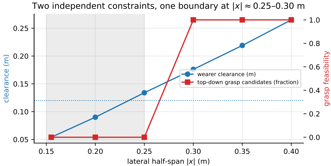
Figure J.5: Wearer clearance and top-down grasp feasibility against lateral half-span. The two constraints were measured independently and for different purposes, and both place the usable boundary at |x| \approx 0.25 to 0.30 m.
