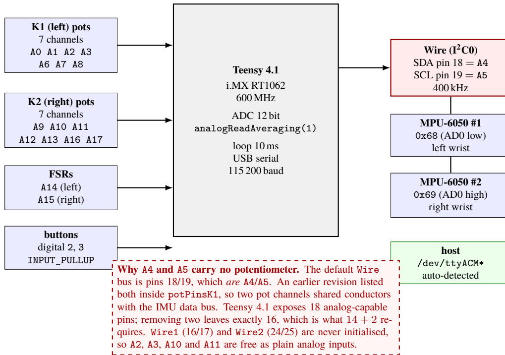
Figure B.3: Electronics architecture and pin assignment. The call-out explains why two analog-capable pins carry no potentiometer.
