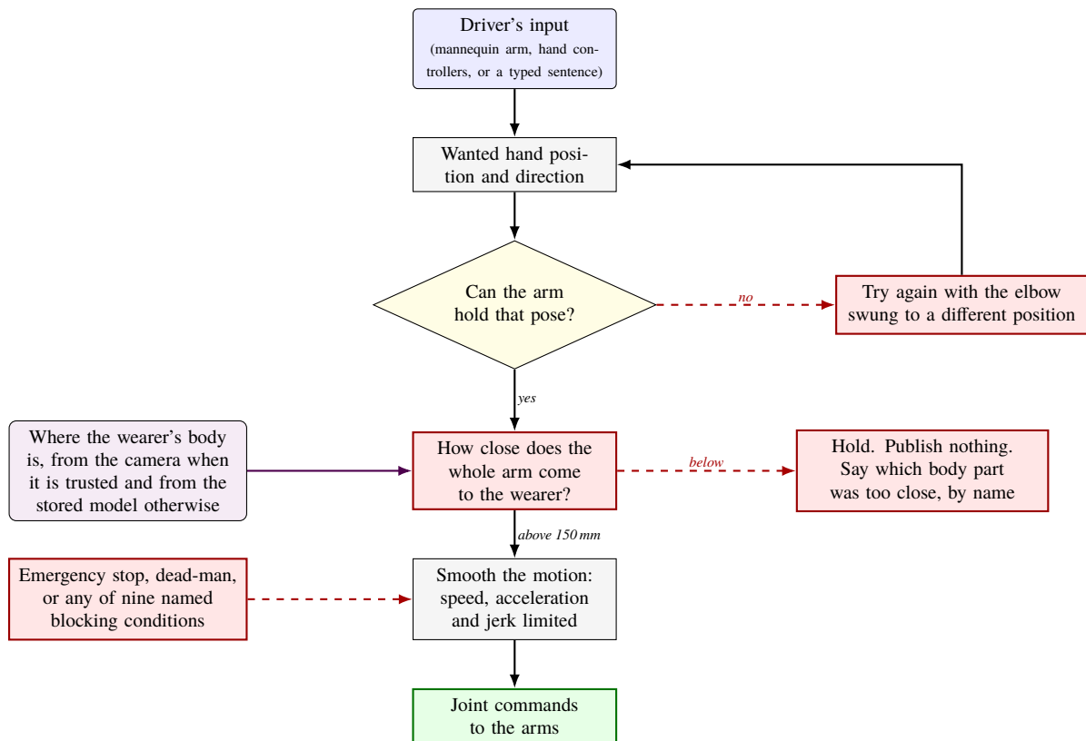
Figure D.2: The path every commanded pose takes, in any mode. Red stages can stop the arm and the green stage is the only one that moves it. The two that matter most are the redundancy re-seed, which recovers poses a single solve would drop, and the clearance stage, which is measured geometrically against the wearer rather than taken from the semantic collision description. The per-mode diagrams later in this chapter expand the top of this path; the bottom of it is identical in all of them.
