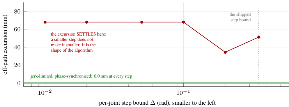
Figure I.1: The excursion is a property of the algorithm, not of its tuning. Sweeping the per-joint step bound over a factor of 35 does not drive the excursion toward zero: it settles at 68 mm, and is in fact worse at small steps than at the shipped one. Section F.1.3 gives the reason — the clamped step is parallel to the required displacement only when every joint is inside the bound or every joint is saturated equally, and at no step size is that generally true. Each point is a genuinely different path densified at 0.02 rad, not one path sampled at different rates.
