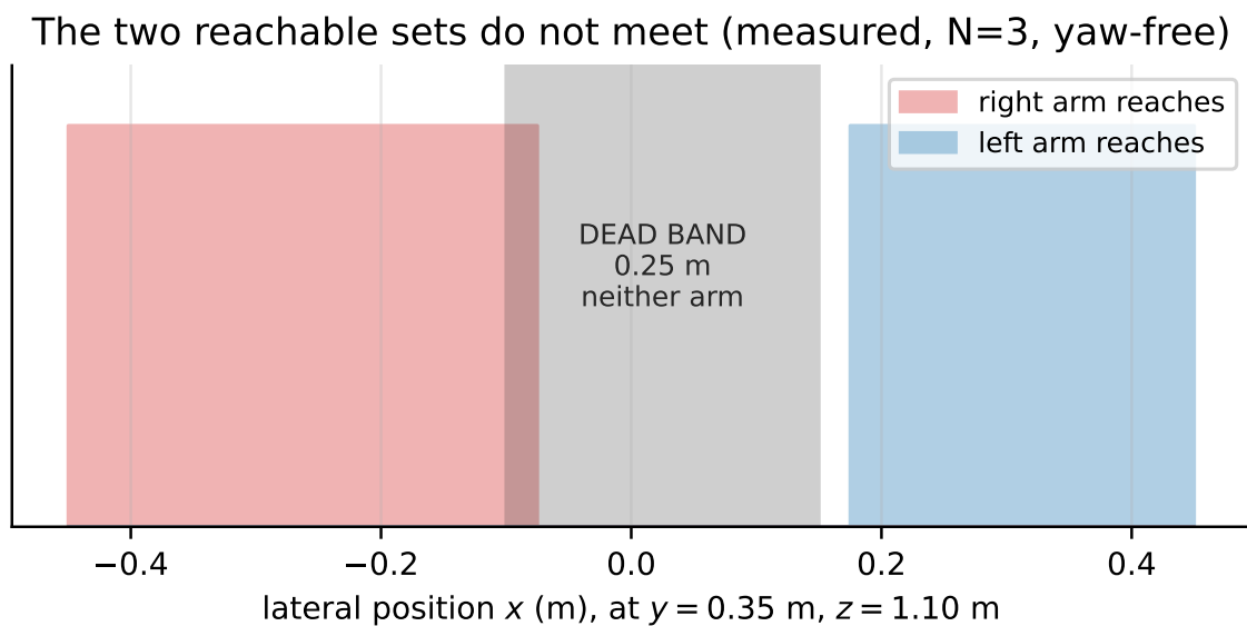
Figure J.3: The two reachable sets do not meet. Measured at y = 0.35 m, z = 1.10 m with yaw free and three repeats per point.
