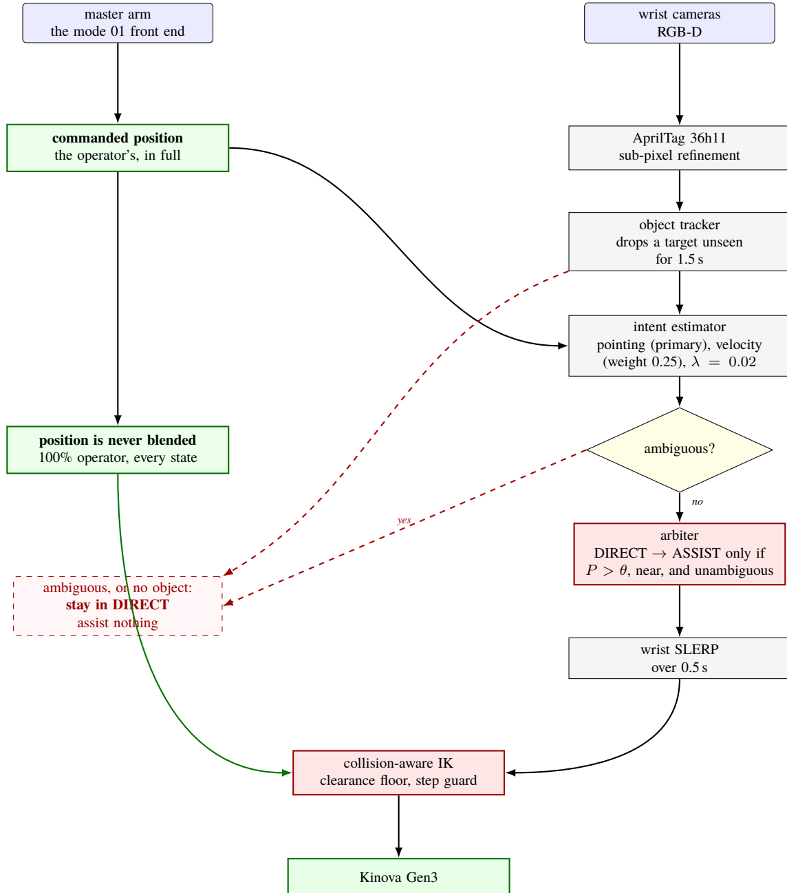
Figure D.6: Mode 04, shared autonomy. The green spine carries commanded position and does not pass through the autonomy stack, so no failure of intent estimation, object tracking or grasp synthesis can move the arm; the autonomy branch reaches only the orientation blend. A tie between two adjacent candidates holds P = 0.5 exactly and the arbiter remains in DIRECT, because assisting toward the wrong one of two candidates is worse than not assisting.
