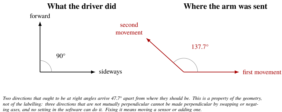
Figure I.6: Two master motions intended to be orthogonal arrive 137.7^\circ apart at the commanded end effector. The test is independent of any axis labelling, which is what makes this a geometric limitation rather than a calibration error.
