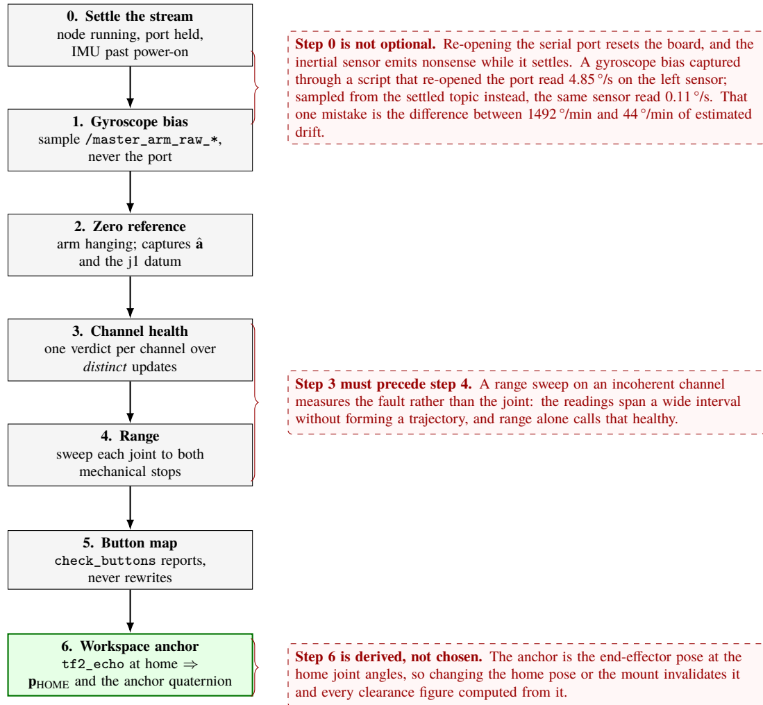
Figure D.11: The calibration procedure, in order. Each step consumes the previous step's output, and the two orderings that are load-bearing are braced to the call-out that explains them. Steps 0 and 3 are both consequences of the same general point: a calibration routine measures whatever the instrument was actually doing at the time, so establishing that the instrument is in a valid state is part of the measurement and not a preliminary to it.
