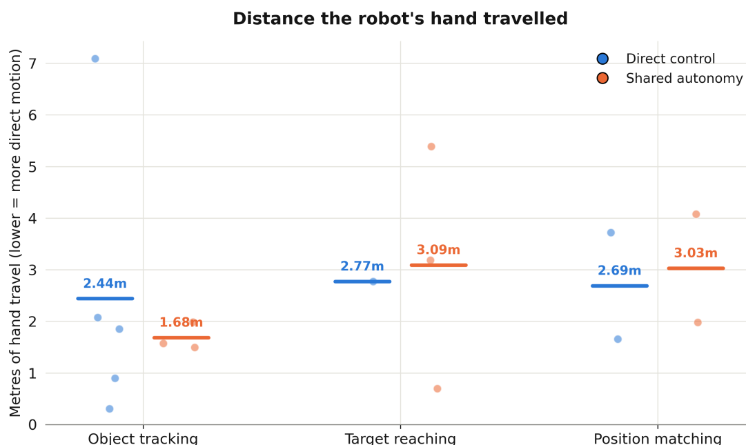
Figure T.1: Distance the robot’s hand travelled, by task and condition. Pooled distance is essentially unchanged between conditions, which is why Section 4.5 reads it as one of the more reliable measures in a pilot where session duration is confounded with setup time.
