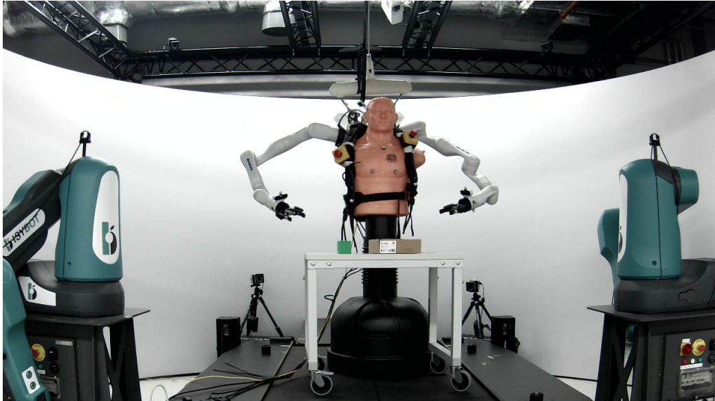
Figure 1.1: The platform as built: two Kinova Gen3 arms on a backpack frame, worn by a torso mannequin, photographed by the room camera. The two teal columns are the laboratory’s fixed robots and are not part of this system.
