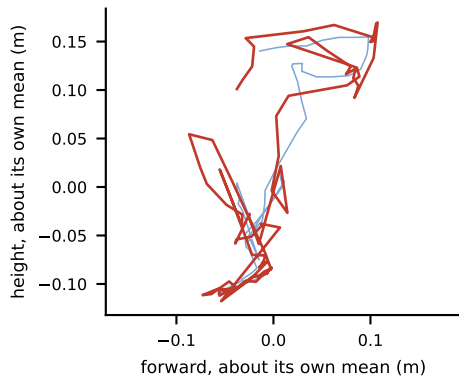
M2, pick and place, direct control
