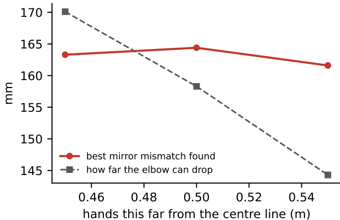
(b) no hand position makes them mirror
