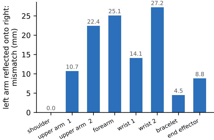
(a) the two arms are not mirror images at home
