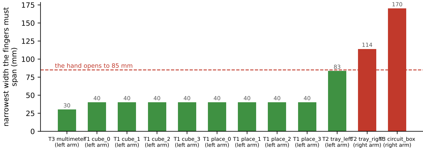
Which task objects fit the hand (green: a grasp was found; red: none)
