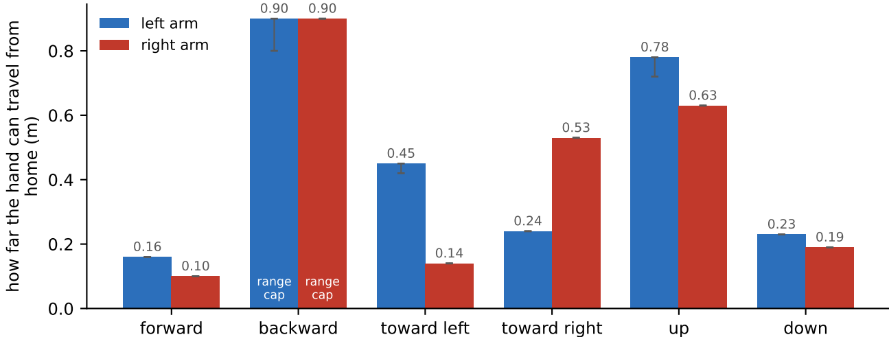
Reach from the home pose, six directions, ten solver repeats each
