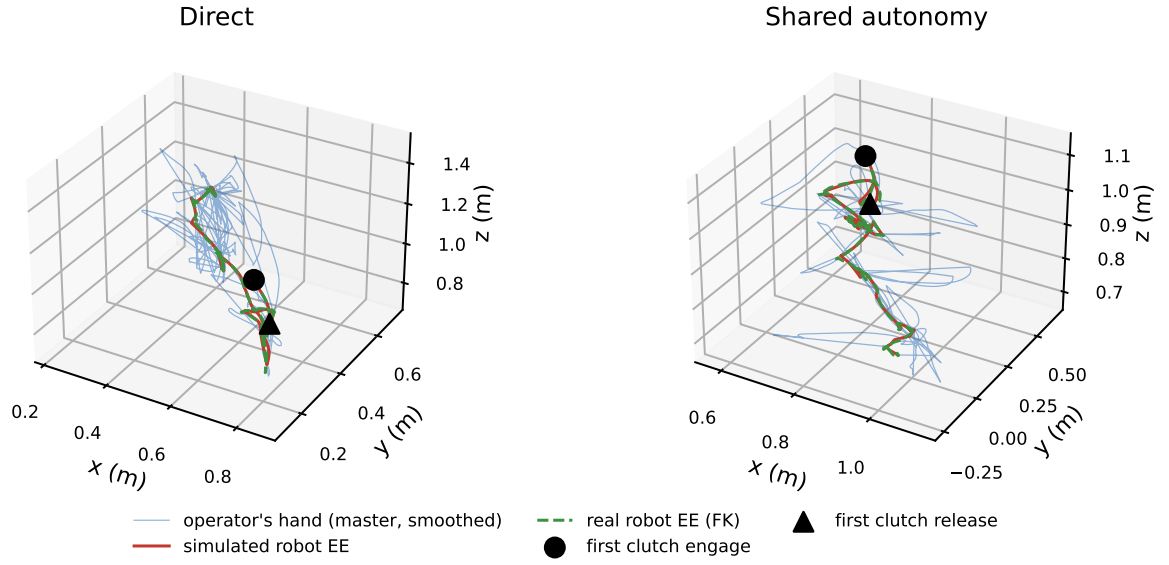
Figure 3.10: VR cohort: master hand (smoothed, the raw input), simulated EE, and the real robot's own EE (forward kinematics on its own encoders) – one Direct and one Shared session, same operator and task, the first clutch engage and release marked. The gripper itself was never commanded in the pilot.
