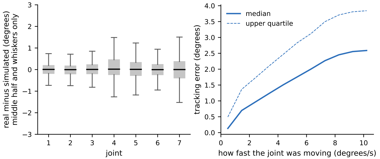
Figure O.8: Pooled over the VR cohort: the error is centred on zero for every joint and grows with joint speed (median 0.13^\circ at rest, 2.59^\circ in the fastest bin) – the real arm lags a moving command rather than sitting off a still one.
