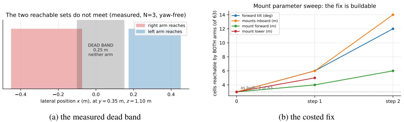
Figure 3.2: (a) The two reachable sets do not meet. (b) A mount-placement sweep: forward tilt and inboard translation help, splaying outward hurts . Kinematic only, so these are upper bounds pending a clearance check.
