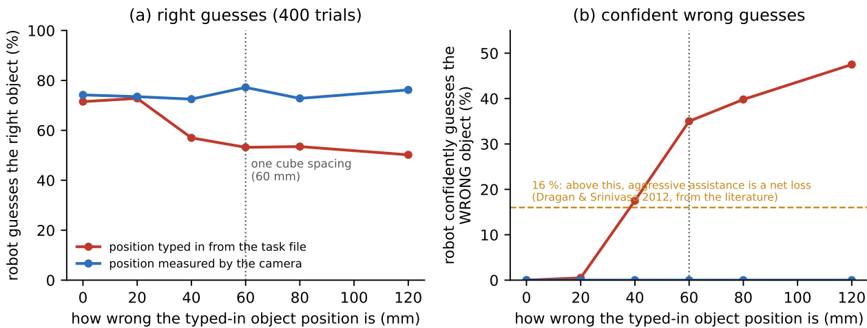
Figure O.27: Four hundred trials per point: from a typed-in object position the estimator's confident wrong guesses climb past the published 16 % break-even at 40 mm of error and reach 35 % at one cube spacing; from the camera's measured position they stay at zero.
