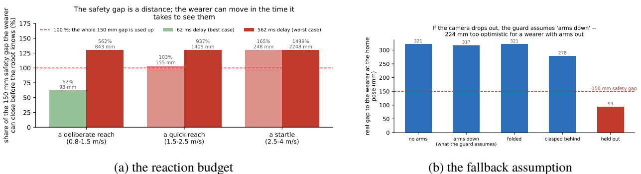
Figure O.25: Left: the share of the 150 mm safety gap a moving wearer closes before the robot knows, three limb-motion classes at the best (62 ms) and worst (562 ms) measured delay. Right: what the guard assumes when the wearer camera drops out (arms down, 317 mm) against a wearer with arms held out (93 mm).
