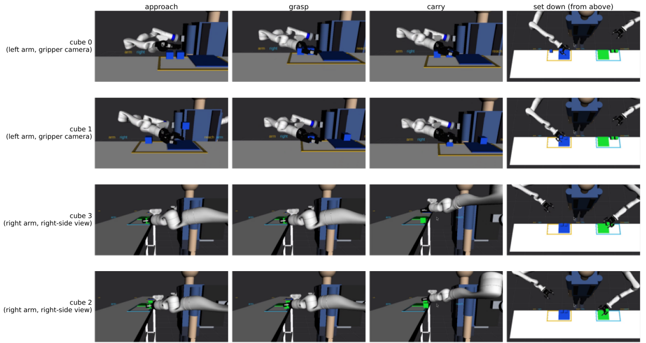
Figure 3.6: The autonomous pick-and-place in simulation, one row per cube: approach, grasp, carry, set-down, cut from the recorded clips at the logged event times; both arms are used.
