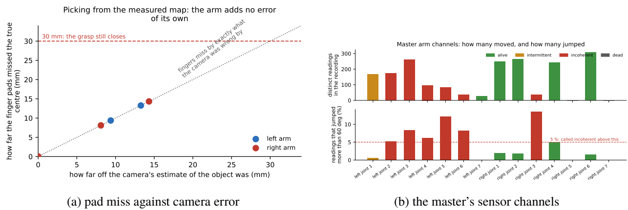
Figure O.30: Left: whatever the camera believes, the arm delivers the fingers there – the pad miss equals the belief error, so the residual is perception, not kinematics. Right: which of the fourteen master-arm sensors read cleanly, the verdict behind Section H.2 .
