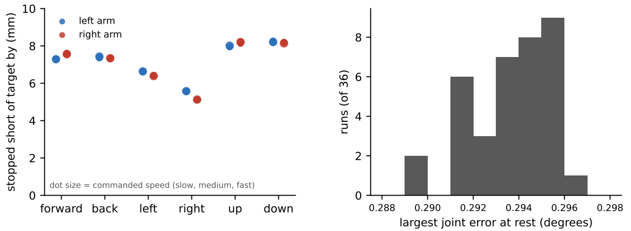
Figure O.23: The thirty-six calibration moves: every 100 mm move stopped 5.1 to 8.3 mm short, the same for both arms and all three speeds, with the worst joint's rest error in a 0.289 to 0.296° band (the pooled per-joint fit in Section E.3 gives 0.305°).
