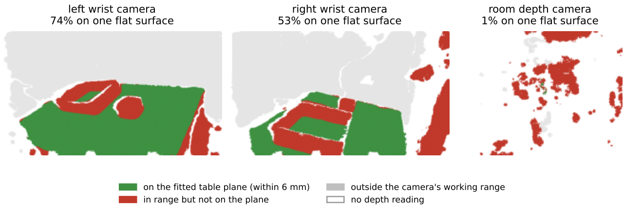
Figure O.19: The support plane the pipeline fitted, recomputed over each camera's own depth array with the stored plane and tolerance: 73.95 % of the left wrist camera's points lie on it, 52.79 % of the right's, and under 1 % of the room depth camera's (the pipeline's own log says 3.75 % for that camera; both mean no usable surface).
