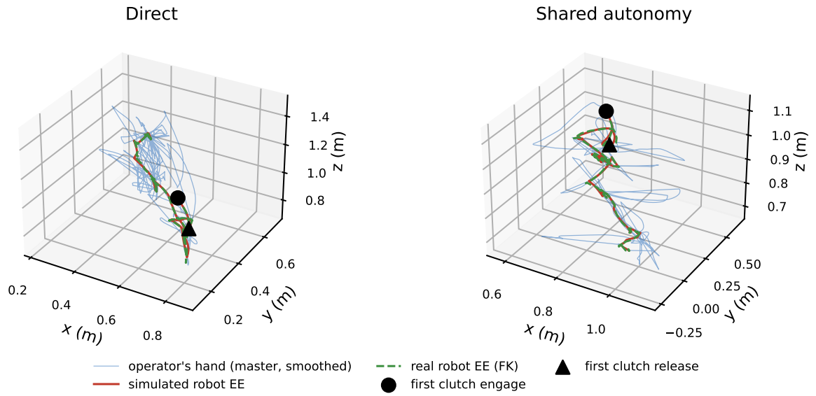
Figure 3.10: VR cohort: master hand (smoothed, the raw input), simulated EE, and the real robot's own EE (forward kinematics on its own encoders) – one Direct and one Shared session, same operator and task, the first clutch engage and release marked. The gripper itself was never commanded in the pilot.
