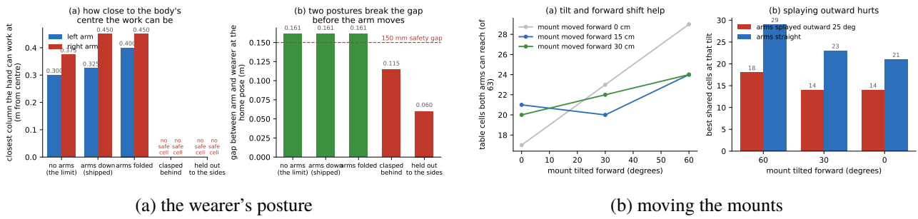
Figure O.29: Left: how the wearer's arm posture changes what the arms can reach, with the 150 mm gap drawn. Right: how moving the mounts changes what both arms can reach – as built the two share three of 63 cells; the buildable best is 22.
