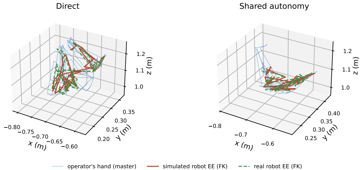
Figure 3.11: The master-arm cohort's own version of Fig. 3.10: M2, Direct and Shared, same task, both under 2.3° sim-to-real RMS. This cohort logs no clutch channel, so no markers are drawn.
