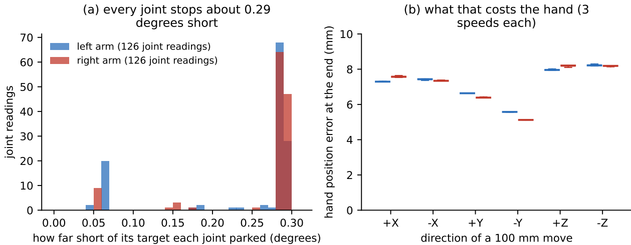
Figure O.26: Thirty-six real moves of 100 mm: every joint stops about 0.29° short (a), which costs the hand 5 to 8 mm by direction, the same at all three speeds (b).
