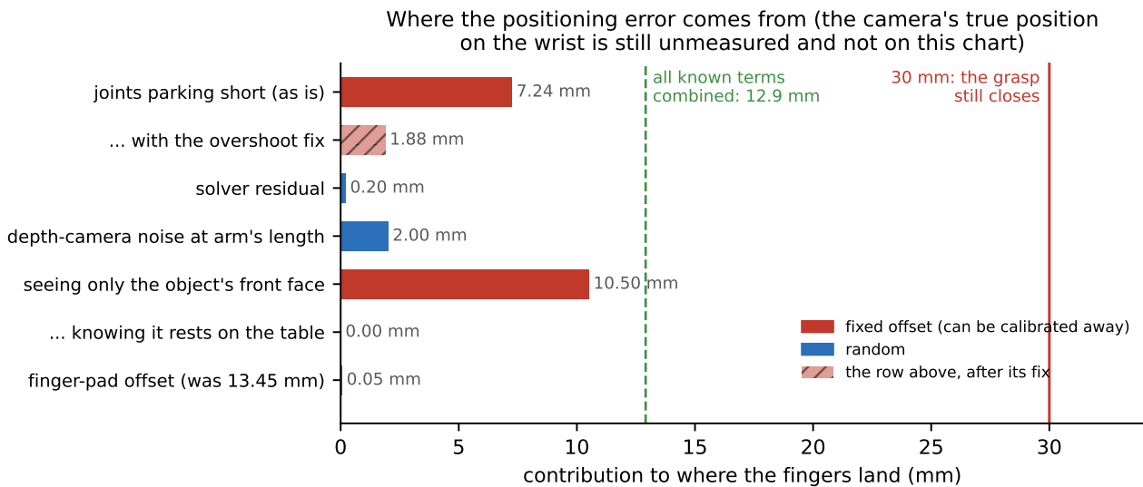
Figure O.24: Each known source of finger-landing error as a bar, fixed offsets distinguished from random terms and each fix shown against the row it fixes; combined 12.9 mm against the 30 mm grasp line. The camera's true position on the wrist is unmeasured and not on this chart.
