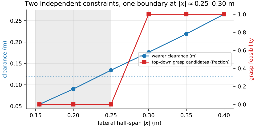
Figure 8.4: Wearer clearance and top-down grasp feasibility against lateral half-span. The two constraints were measured independently and for different purposes, and both place the usable boundary at |x| \approx 0.25 to 0.30 m.
