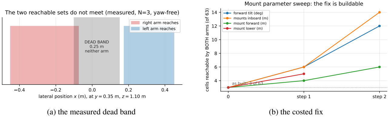
Figure 4.1: (a) The two reachable sets do not meet. (b) A mount-placement sweep: forward tilt and inboard translation help, splaying outward hurts . Kinematic only, so these are upper bounds pending a clearance check.
