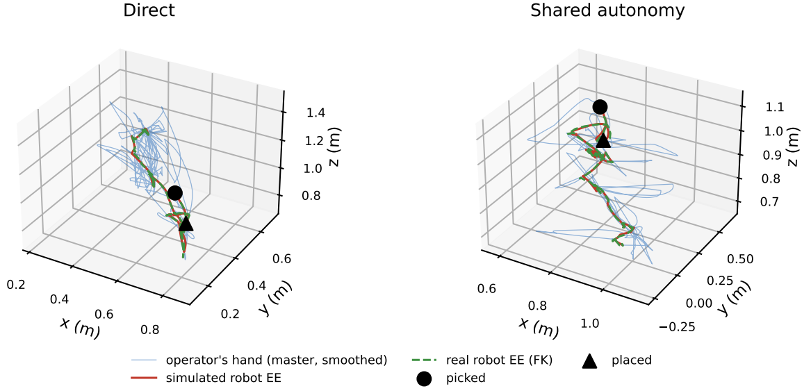
Figure 4.6: VR cohort: master hand (smoothed, the raw input), simulated EE, and the real robot's own EE (forward kinematics on its own encoders) – one Direct and one Shared session, same operator and task, picked/placed from the gripper's logged transitions. Simulated and real agree closely, the same small gap as Fig. 4.8.
