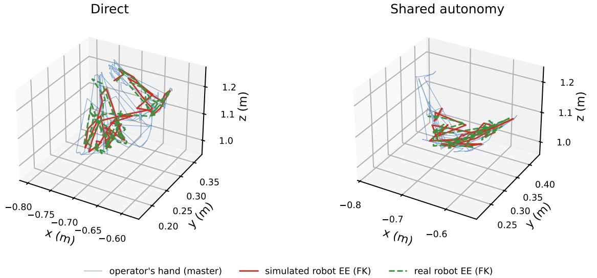
Figure 4.7: The master-arm cohort's own version of Fig. 4.6: M2, Direct and Shared, same task, both under 2.3^\circ sim-to-real RMS. This cohort logs no gripper channel, so no picked/placed markers are drawn.
