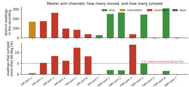
(b) the master's sensor channels
