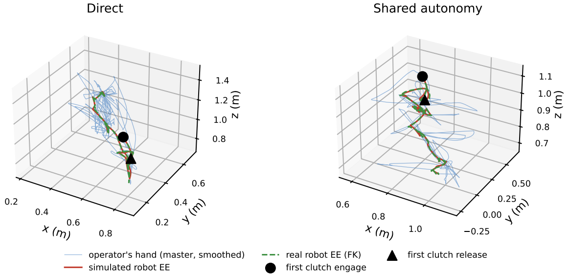
Figure 3.10: One VR operator, one direct and one assisted session of the same task: the operator's hand (smoothed), the simulated robot's hand, and the real robot's hand computed from its own joint encoders; the first clutch press and release are marked. The gripper itself was never commanded in the pilot.
