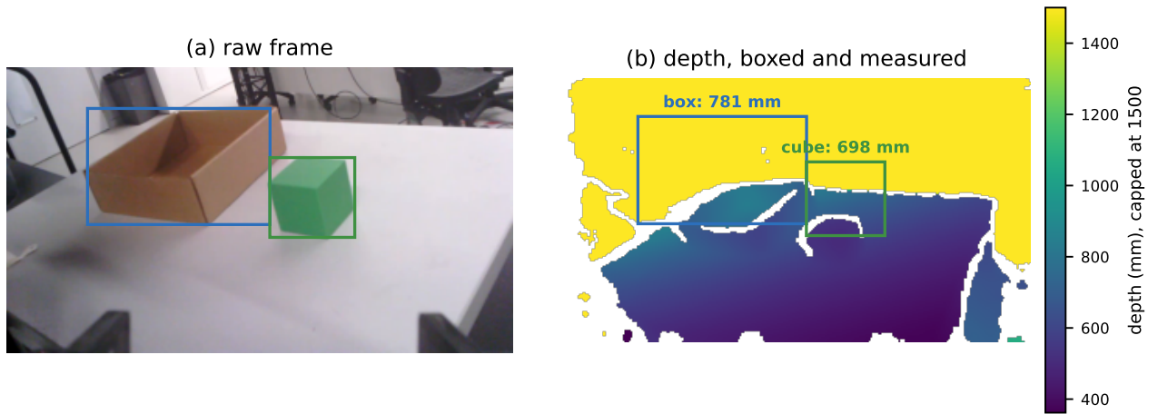
Figure 3.4: Figure 3.3’s frame (a) beside its depth map (b), each object boxed and labelled with its median measured distance.
