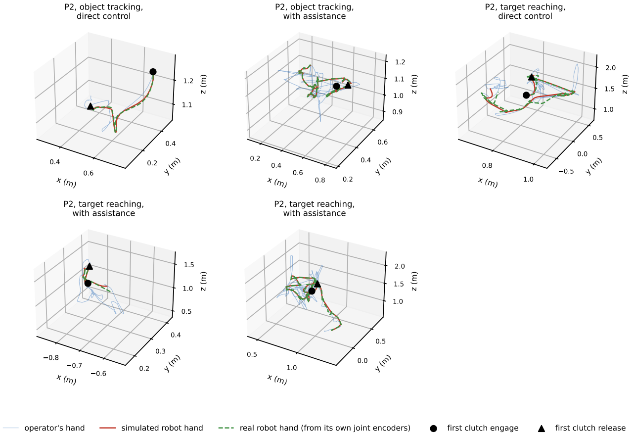
Figure O.19: Every recorded session of P2: the operator's hand (faint, smoothed), the simulated robot's hand and the real robot's hand from its own encoders.
