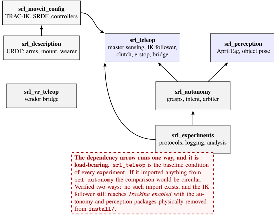
Figure 2.1: The software packages and their one-way dependencies: the teleoperation package, the baseline condition of every planned experiment, imports nothing from the autonomy package – verified by inspecting the source and by running it with the autonomy and perception packages deleted.
