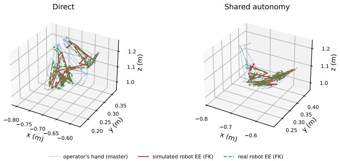
Figure 3.11: The mannequin-master cohort's version of Fig. 3.10: M2, direct and assisted, same task, both under 2.3^\circ of joint tracking error. This cohort logs no clutch channel, so no markers are drawn.
