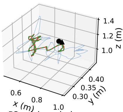
P3, pick and place, direct control
