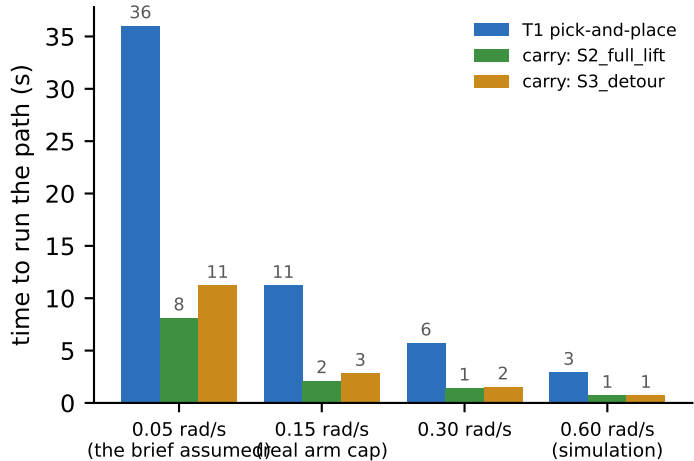
(a) the real speed cap makes a pick take 11 s
