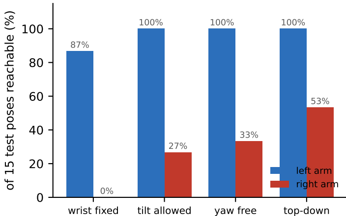
(b) the right arm reaches little with a fixed wrist
