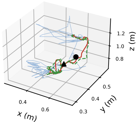
P1, pick and place, direct control
