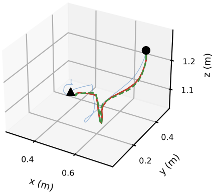
P2, pick and place, direct control (gap 14 mm)
