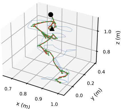
P5, pick and place, with assistance (gap 12 mm)
