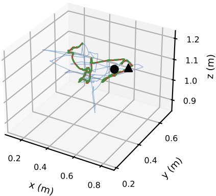
P2, pick and place, with assistance (gap 9 mm)
