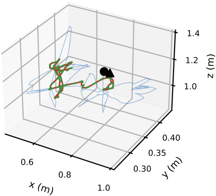
P3, task not labelled, with assistance (gap 7 mm)
