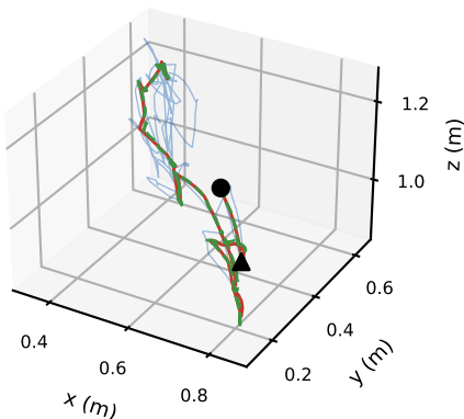
P5, pick and place, direct control (gap 11 mm)
