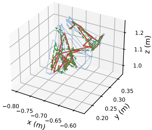
Direct
