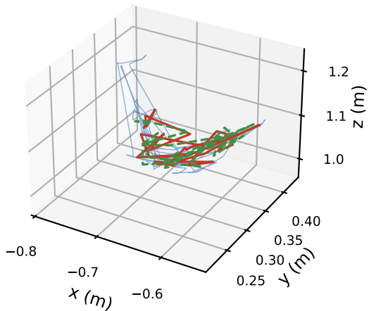
Shared autonomy
