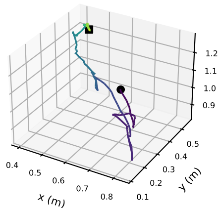
M2, mannequin master: 9.20 m in 302 s
