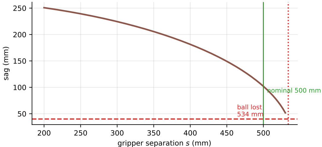
Compliant sling: nonlinear failure, L = 540 mm, r = 20 mm
