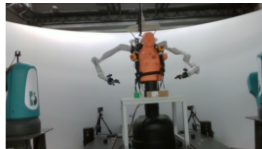
Room depth camera RGB-D (RealSense D435i)
