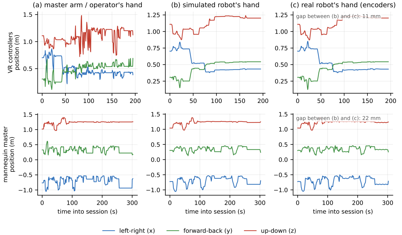
Figure 4.10: Where each hand was, second by second, for one session per cohort: (a) the master arm or operator's hand, (b) the simulated robot's hand as RViz shows it, (c) the real robot's hand from its own joint encoders. Top: VR (P4, pick and place, direct). Bottom: mannequin master (M2, target reaching, direct). Panels (b) and (c) share a scale and are near-identical – the real arm follows the simulation to 11 and 22 mm; the operator's hand (a) moves more, because the mapping scales and filters it.
