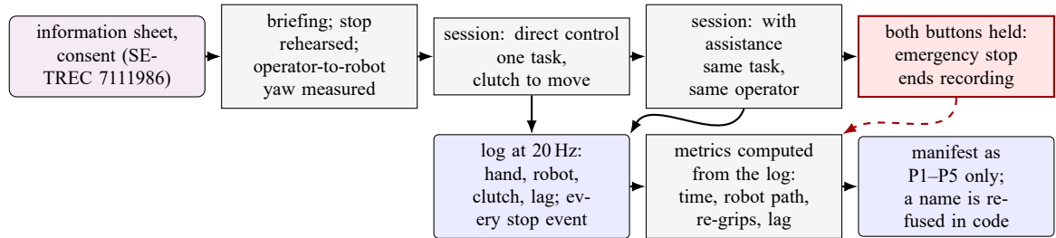
Figure 3.4: One pilot session as run, and the record every metric came from; nothing was timed by hand, and the stop that ends a recording is itself in the log (twelve holds, eleven sessions).
