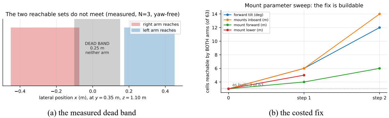
Figure 4.2: (a) The two arms' reachable regions do not meet. (b) Sweeping the mount position: tilting forward and moving inboard help, splaying outward hurts . Geometry only, so these are upper bounds pending a clearance check.
