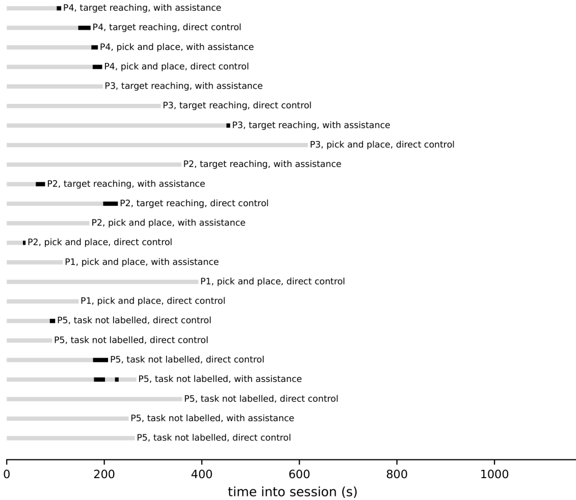
Figure 4.1: Every VR pilot session as a bar, emergency-stop holds in black: twelve holds in eleven sessions; the automatic clearance floor never fired.
