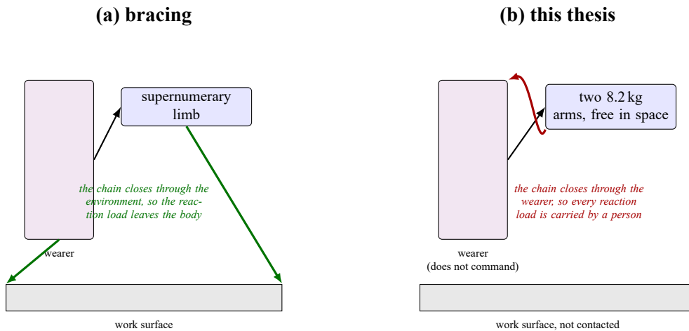
Figure M.1: Bracing (the field's founding configuration [5]) against free-space mounting (this platform).
