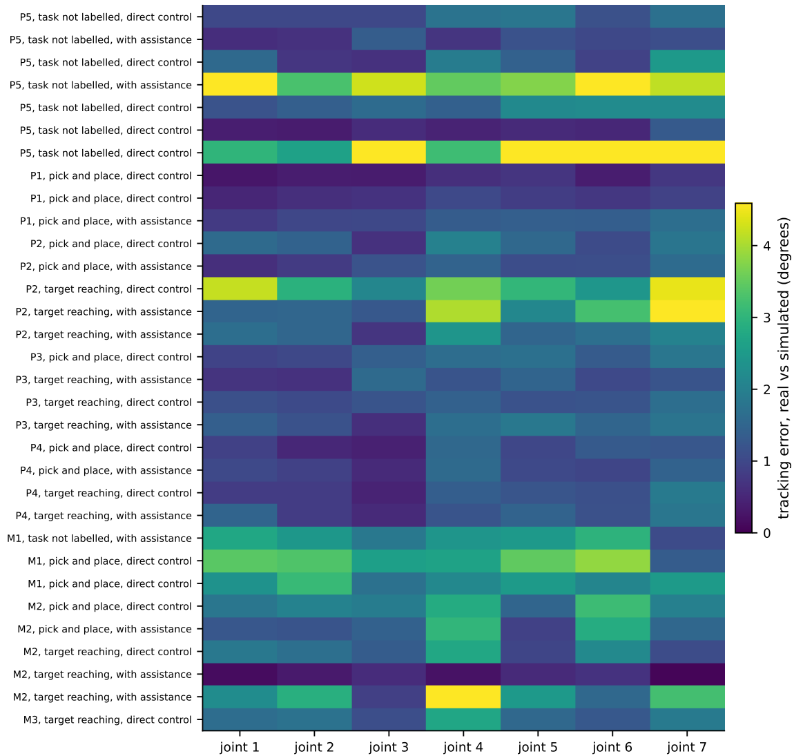
Figure O.7: How closely the real arm followed the simulated one, every session (rows) by joint (columns), both cohorts. Median per-joint error 1.44°; the three M1 rows and two P5 rows light up on several joints at once, the signature of a bad input channel rather than a bad joint; every P1–P4 session stays under 4.6° on every joint.
