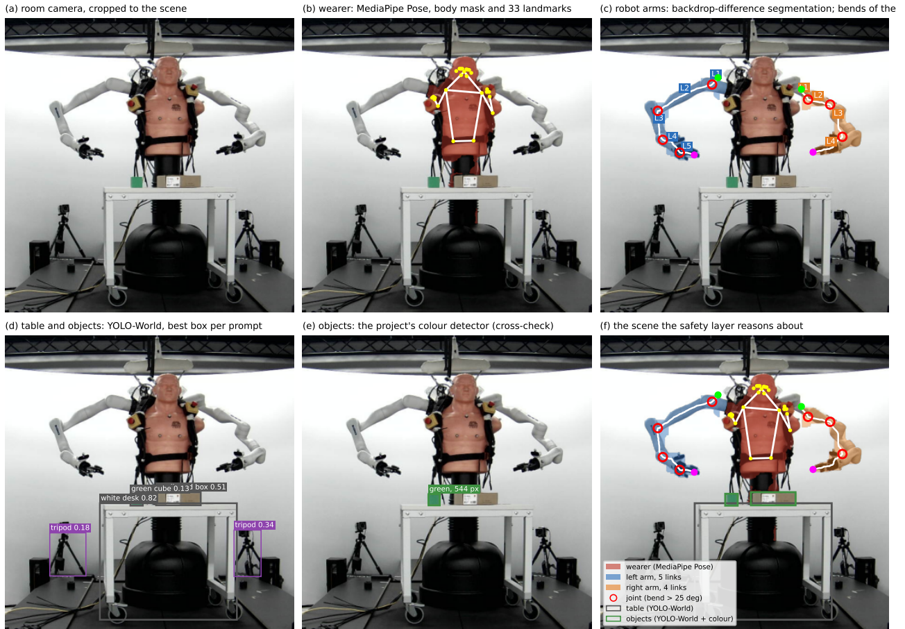
Figure F.1: The room camera's frame, cropped to the wearer, the arms and the table, read by three methods. (b) The wearer by MediaPipe Pose: body mask and 33 landmarks. (c) The robot arms by a backdrop-difference rule, thinned to a centreline with a joint wherever it bends by more than 25°: five links on the left arm, four on the right. (d) The table and objects by YOLO-World with descriptive prompts; (e) the project's colour detector as a cross-check. (f) All of it on one frame. Every mask, landmark, box and score is the method's own output (figures/make_scene_understanding.py).
