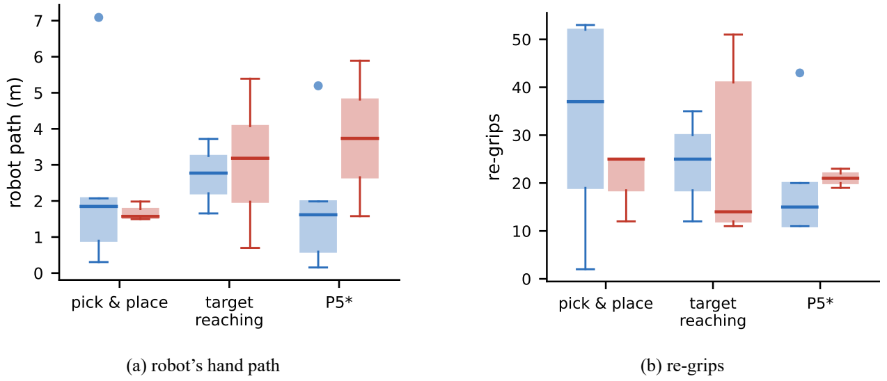
Figure 4.9: The counter-intuitive half of Table 4.3 : with assistance the robot's path is longer in two of three task groups, while re-grips fall.
