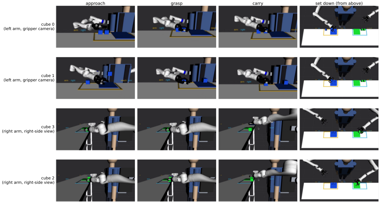
Figure 4.6: The autonomous pick-and-place in simulation, one row per cube: approach, grasp, carry and set-down, at the logged event times; both arms are used.
