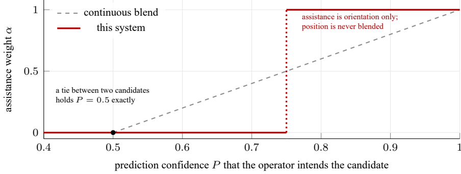
Figure 3.2: The rule this system uses to decide when the robot assists, plotted from its own settings, beside the continuous blend it deliberately does not use.
