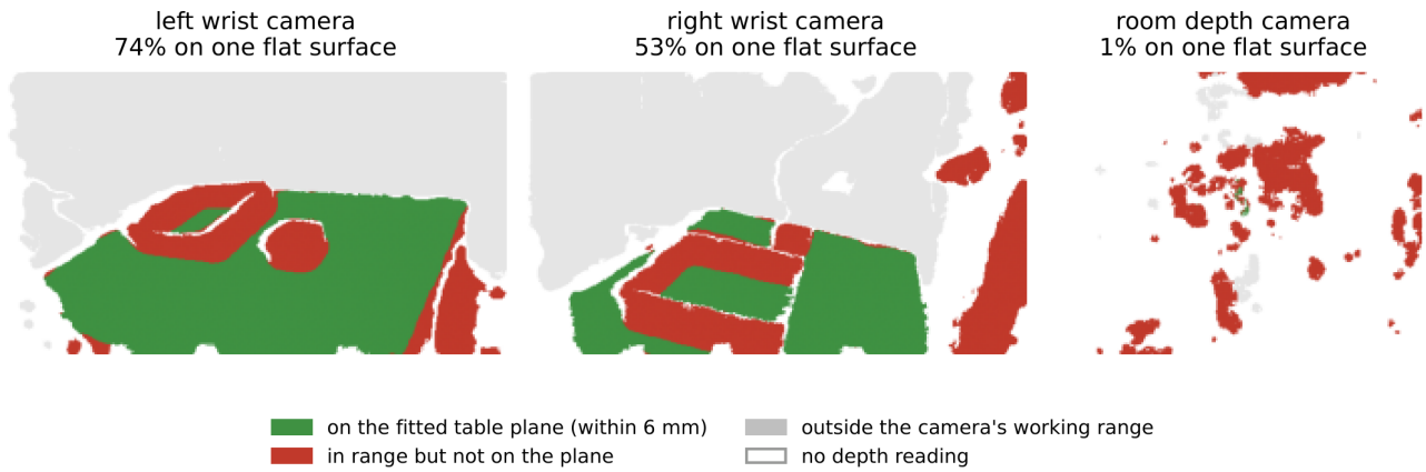
(a) where each depth camera found the flat table
