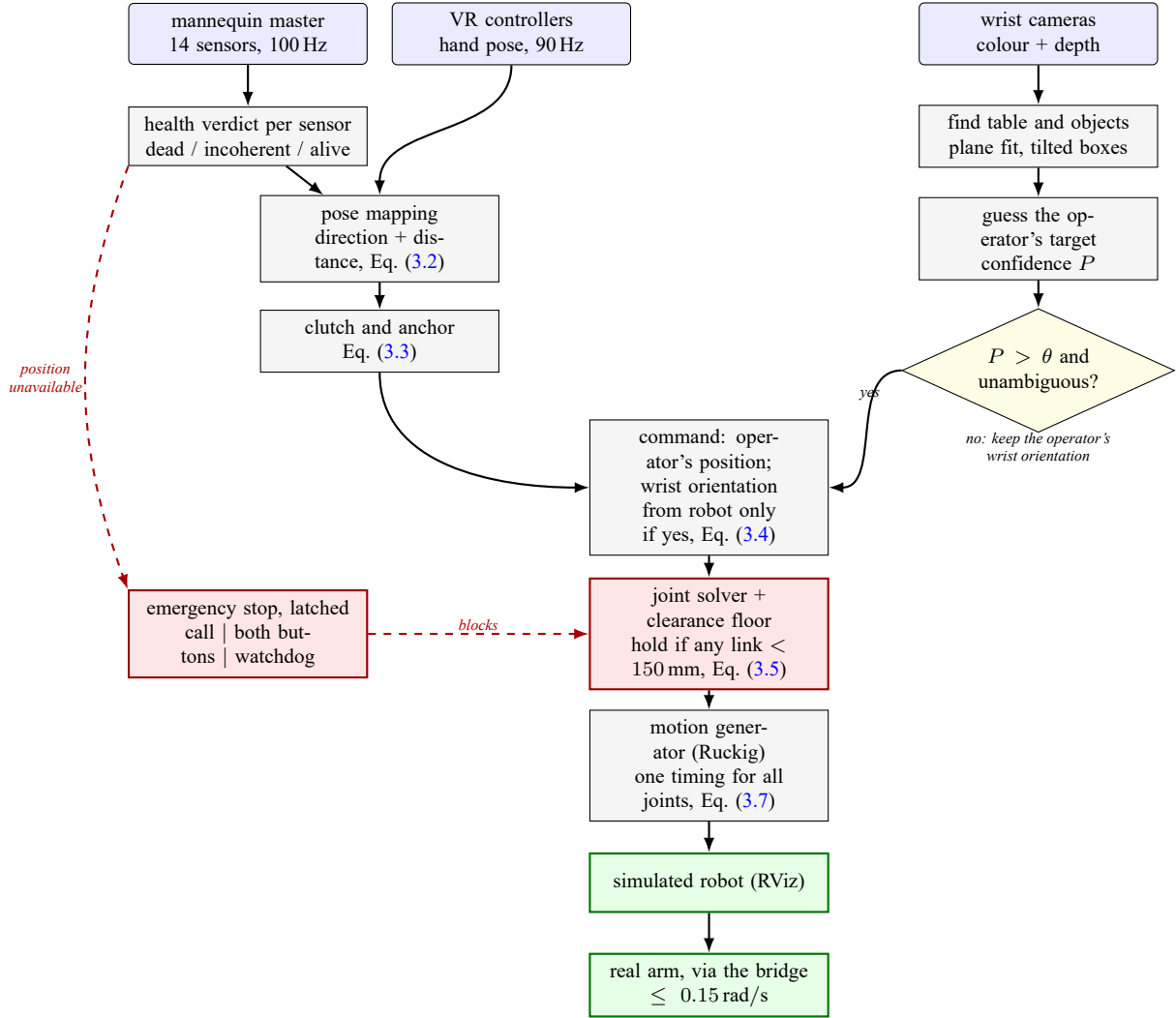
Figure 3.1: The signal path from the operator’s input to the real arm, with every point at which something can stop the arm in red. The operator’s position always passes straight through; the robot may supply the wrist orientation only.
