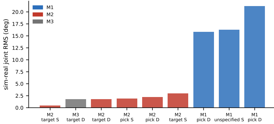
Figure L.4: Sim-to-real joint tracking error for every recorded master-arm session, sorted low to high. M2 and M3 track within 3° throughout; every one of M1’s three sessions tracks an order of magnitude worse (15.9 to 21.2°).
