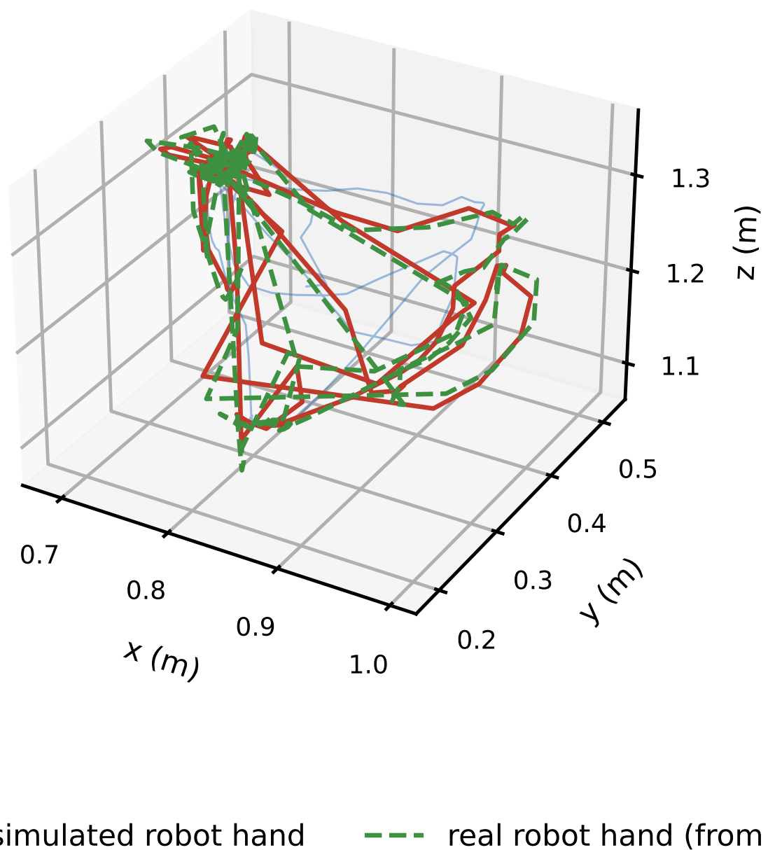
Figure O.25: Every recorded session of M3: the operator's hand (faint, smoothed), the simulated robot's hand and the real robot's hand from its own encoders.
