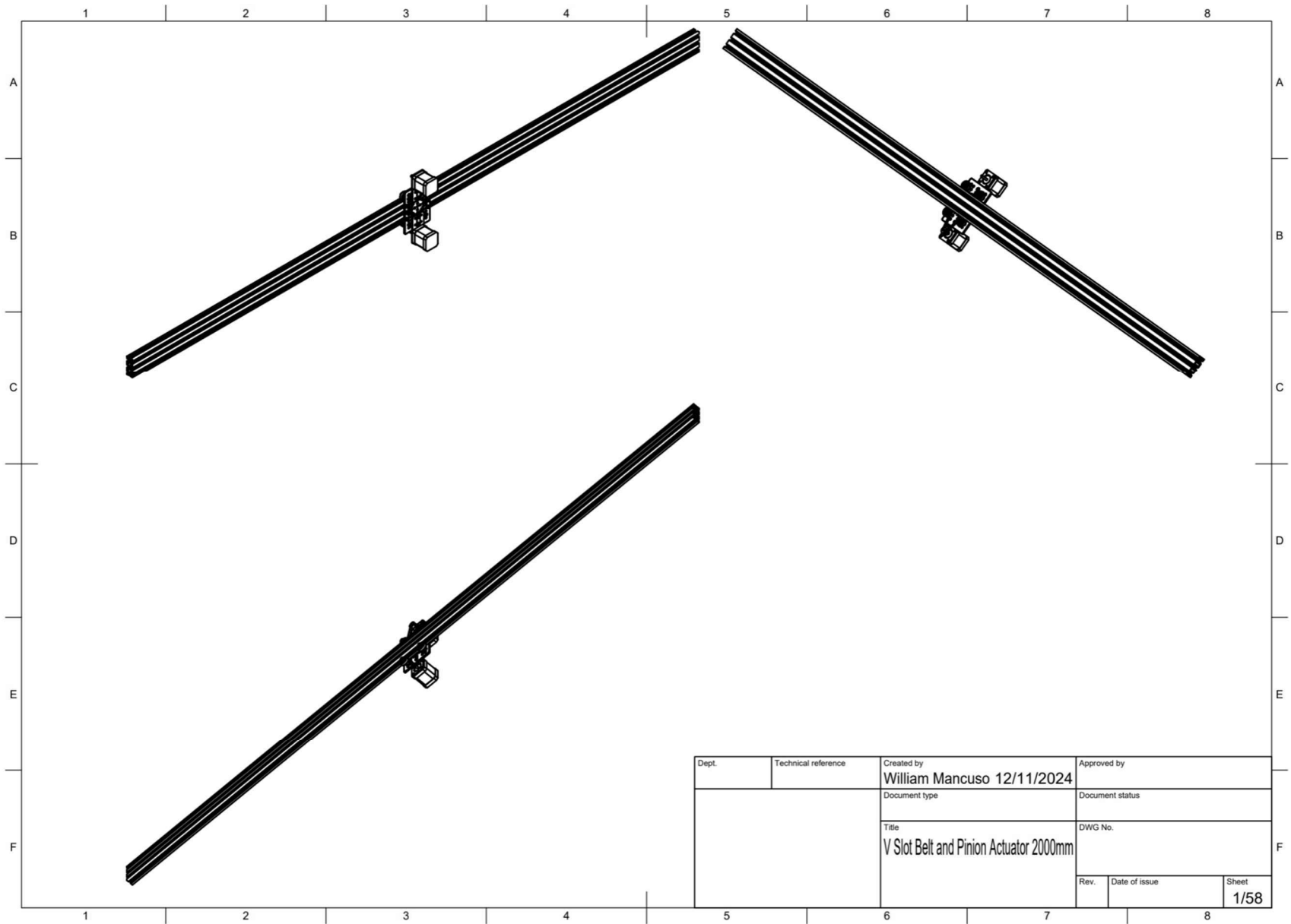
Figure 0-13: Manufacturing Drawing of part SS#2-P#1- Linear Actuators
