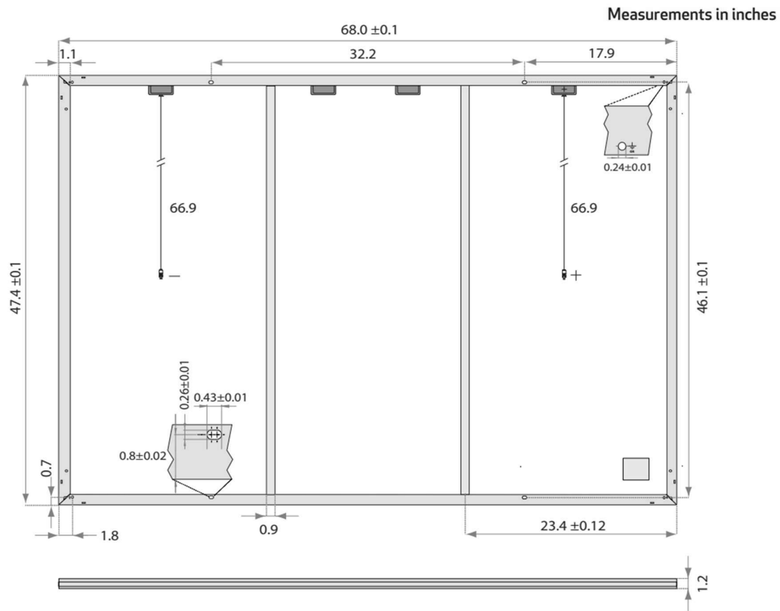
Figure 0-4: Manufacturing Drawing of part SS#1-P#1 – Solar Panel
