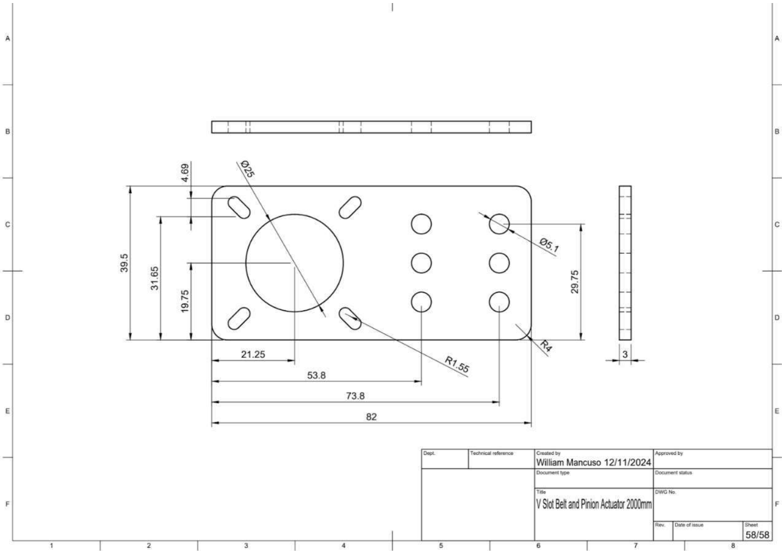
Figure 0-10: Manufacturing Drawing of part SS#2.1-P#2 – Secondary Gantry Plate
