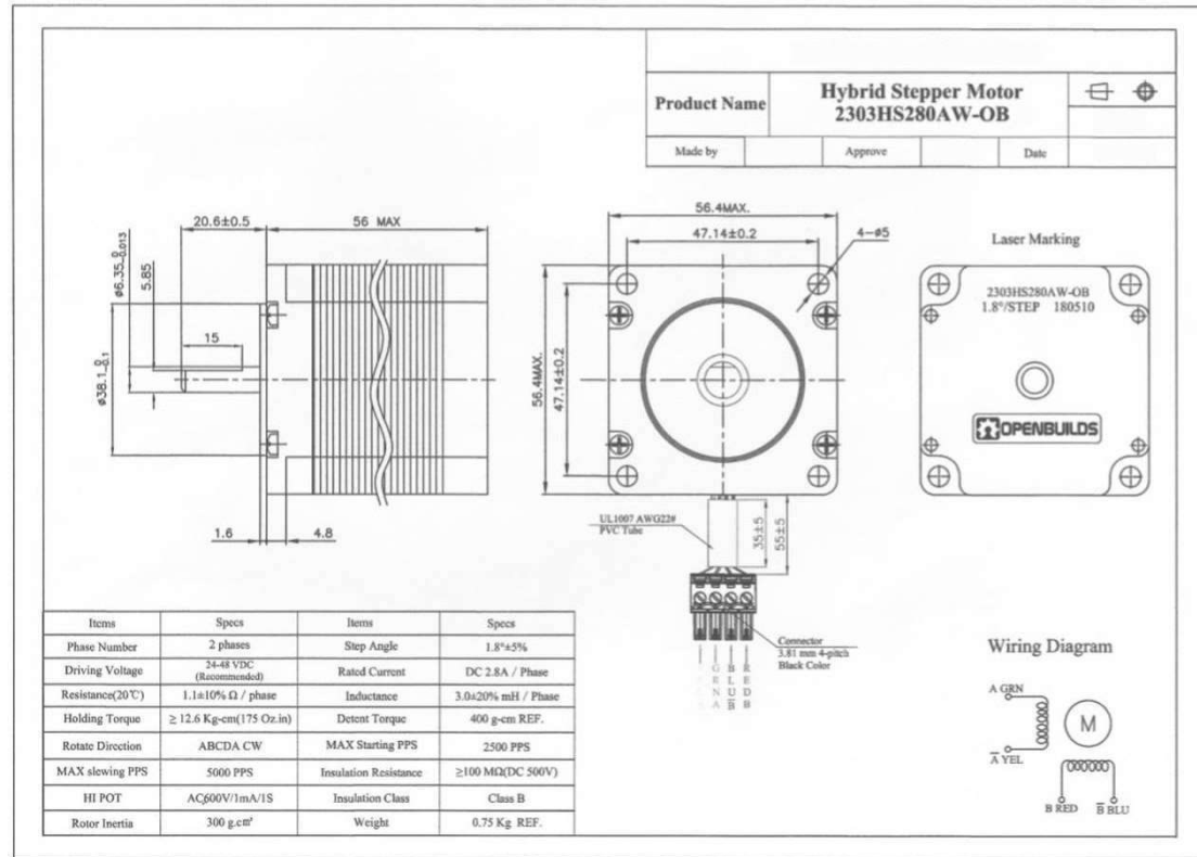
Figure 0-6: Manufacturing Drawing of part SS#2-P#2 – NEMA 23 Stepper Motor
