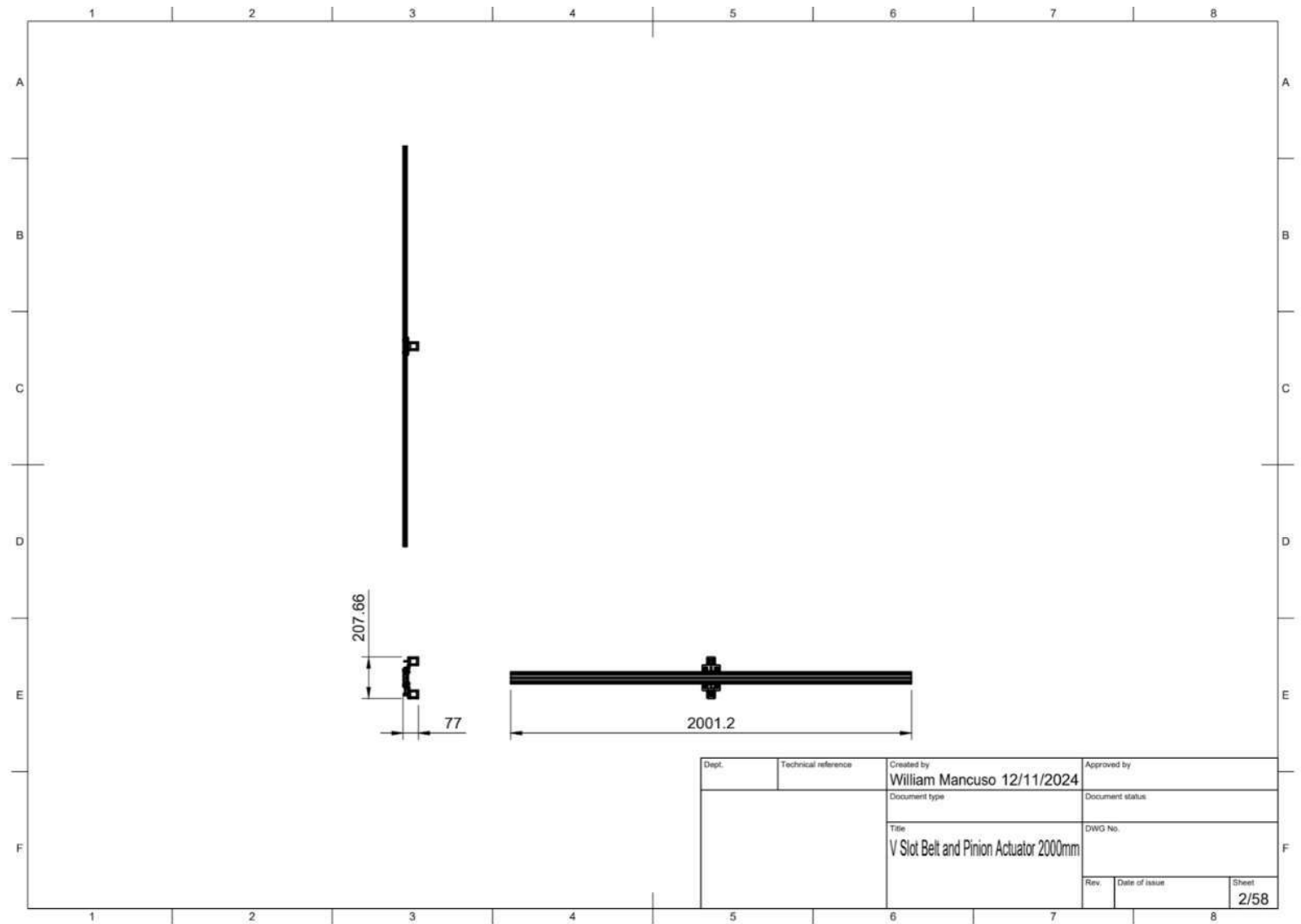
Figure 0-12: Manufacturing Drawing of part SS#2-P#1 - Linear Actuators
